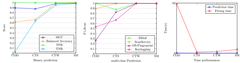
Figure 6: Comparison of spectral graph approaches with baseline on Botnet dataset
