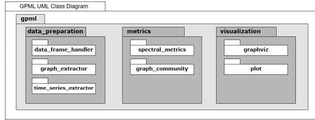
Figure 1: UML diagram showing the structure of the GPML library
