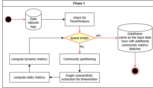
Figure 2: UML workflow diagram community strategy
