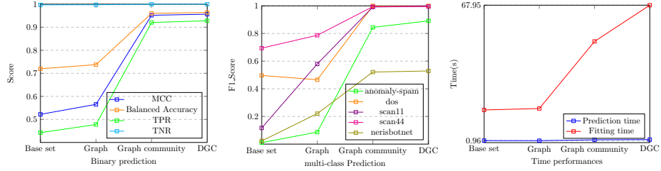
Figure 5: Comparison of graph community approaches with baseline on UGR16 dataset with 5-folds evaluation using XGboost. Base set is original dataset feature space, the other one are the same dataset enriched with incrementally: graph metrics, graph community metrics and dynamic graphe community metrics.
