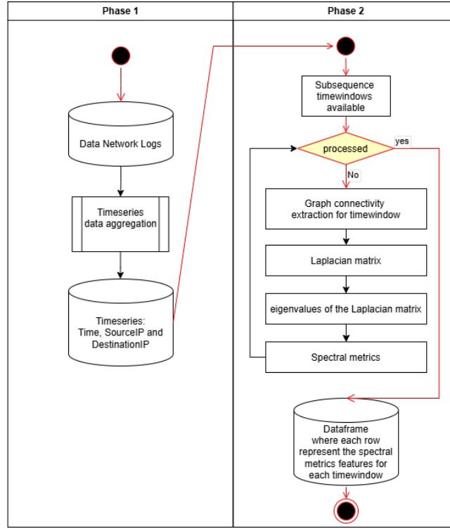
Figure 3: UML workflow diagram for spectral graph strategy
