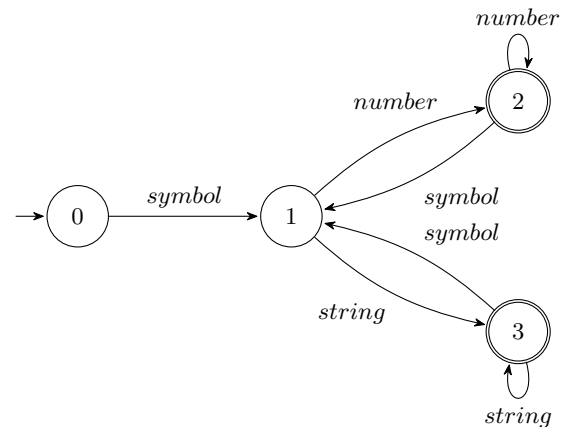
Figure 5: Example DFA
