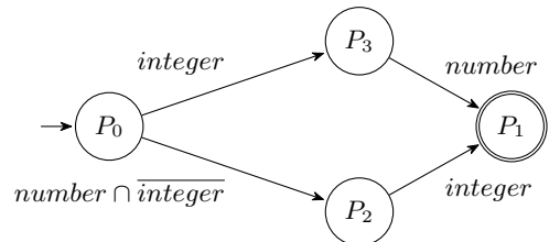
Figure 7: Example DFA with disjoint types
