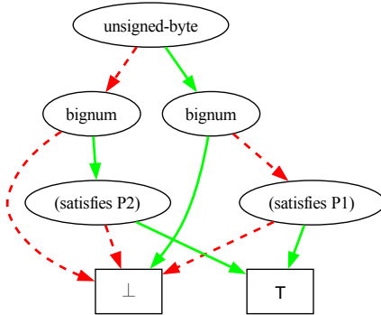
Figure 3: ROBDD with temporary valid satisfies types
