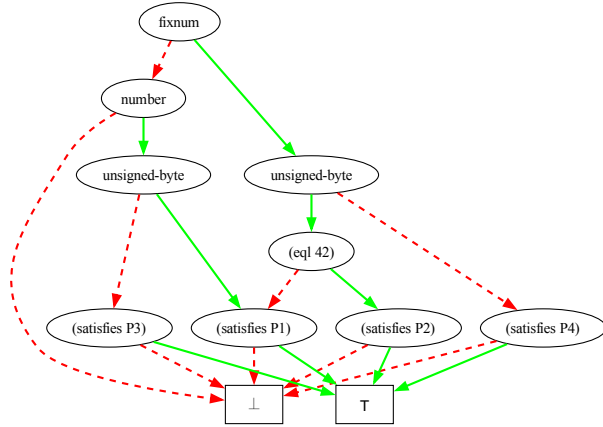
Figure 4: ROBDD generated from typecase clauses in Example 3.4
