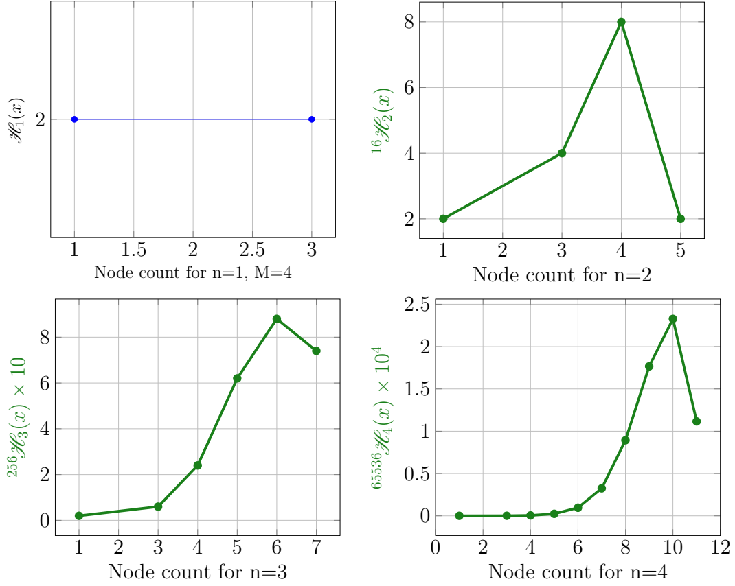
Figure 6.3: Histograms illustrating size distributions of ROBDDs from 1 to 4 Boolean variables. The histograms are based on exhaustive data.
