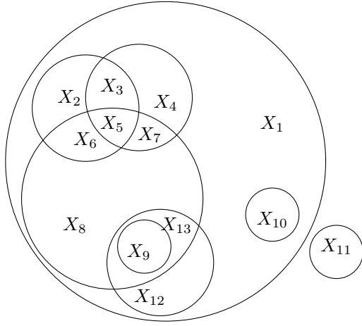
Figure 8.2: Venn Diagram after Decomposition. Each X_i is represented by a region which does not overlay any other region.
