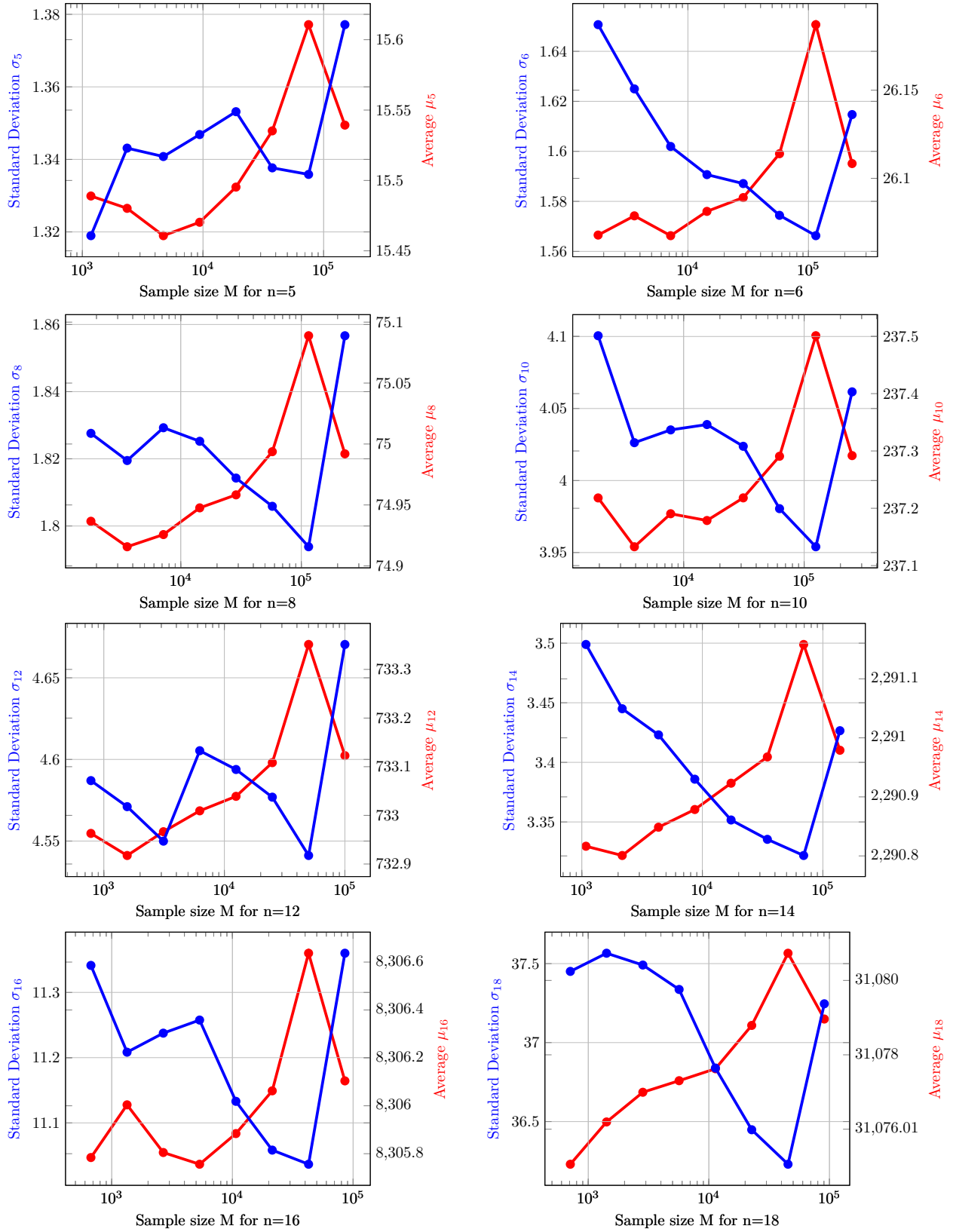
Figure 6.16: Averages ( \mu_n ) and Standard deviations ( \sigma_n ) of the 5, 6, 8, 10, 12, 14, 16, and 18 variable distributions vs. sample size, M .
