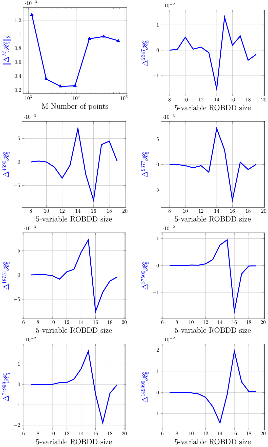
Figure 6.23: Difference functions for n = 5
