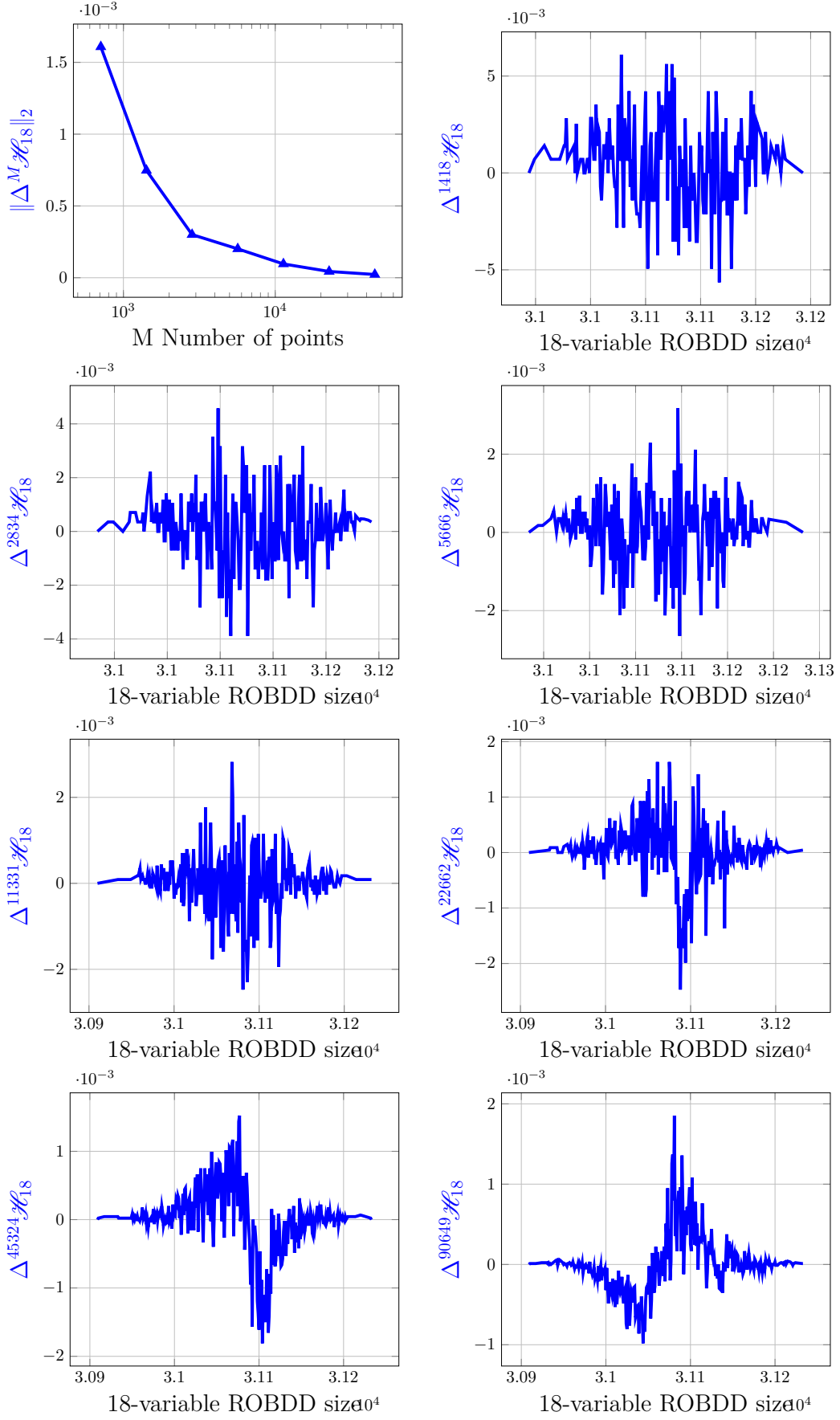
Figure 6.27: Difference functions for n = 18
