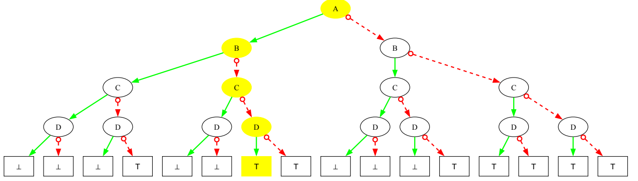
Figure 5.2: UOBDD for F = \neg ((A \wedge C) \vee (B \wedge C) \vee (B \wedge D)) . The highlighted path of nodes corresponds to the highlighted row of the truth table in Figure 5.3.
