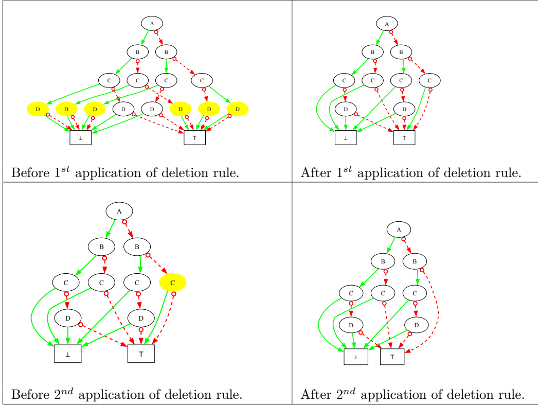
Figure 5.6: Examples of Deletion Rule. The highlighted nodes are symmetric. Such nodes are deleted.
