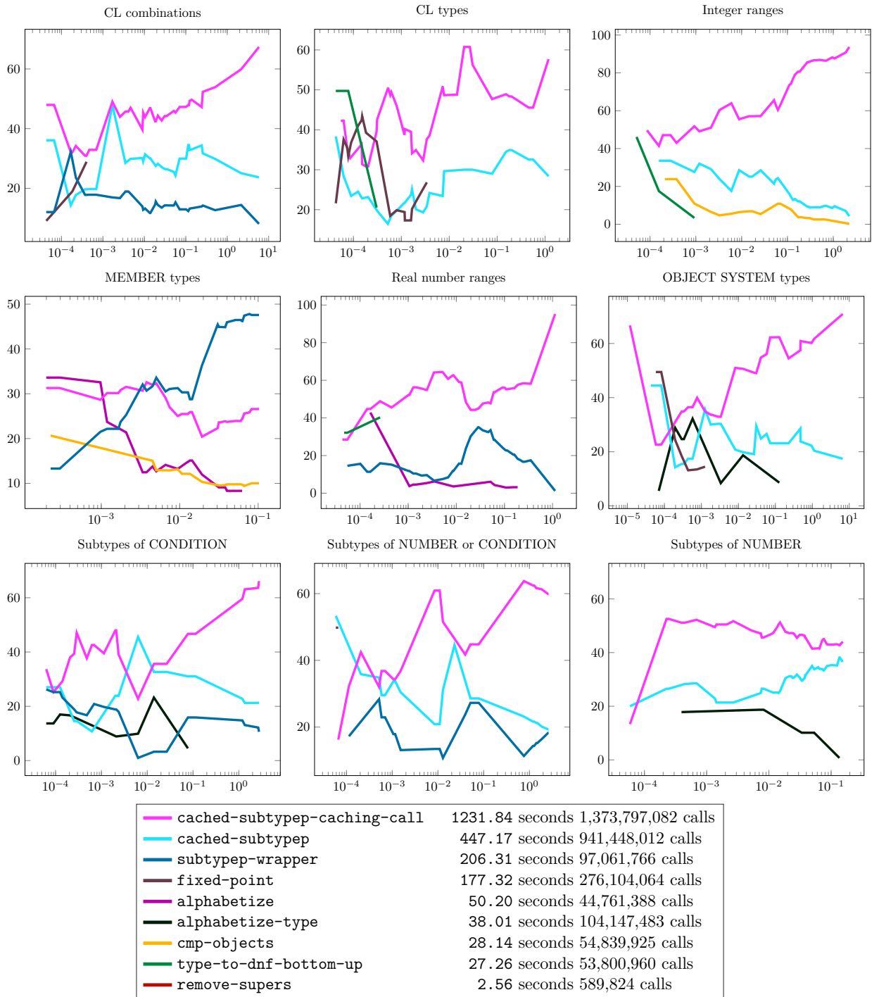
Figure 10.19: Performance Profile of various pools on algorithm mdtd-baseline . Each plot is displayed with y ='Profile Percentage' vs. x ='Computation Time (seconds).'
