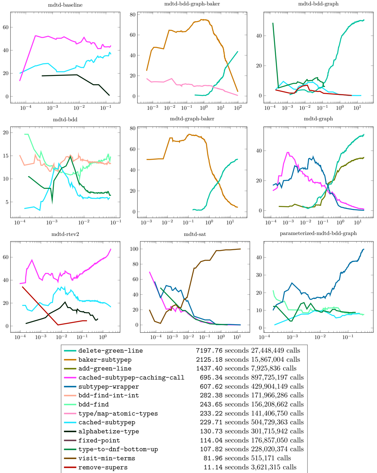
Figure 10.27: Performance Profile of various MDTD functions for pool Subtypes of NUMBER . Each plot is displayed with y='Profile Percentage' vs. x='Computation Time (seconds).'
