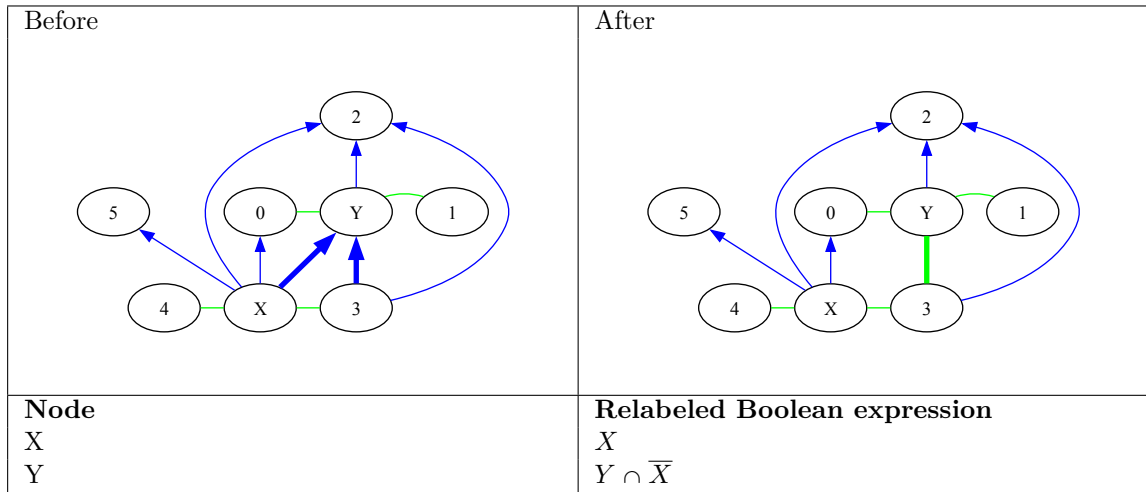
Figure 9.7: Relaxed subset before and after mutation. The blue arrow from X to Y has been eliminated, and the blue arrow from 3 to Y has been converted to a green line because X and 3 are connected with a green line.
