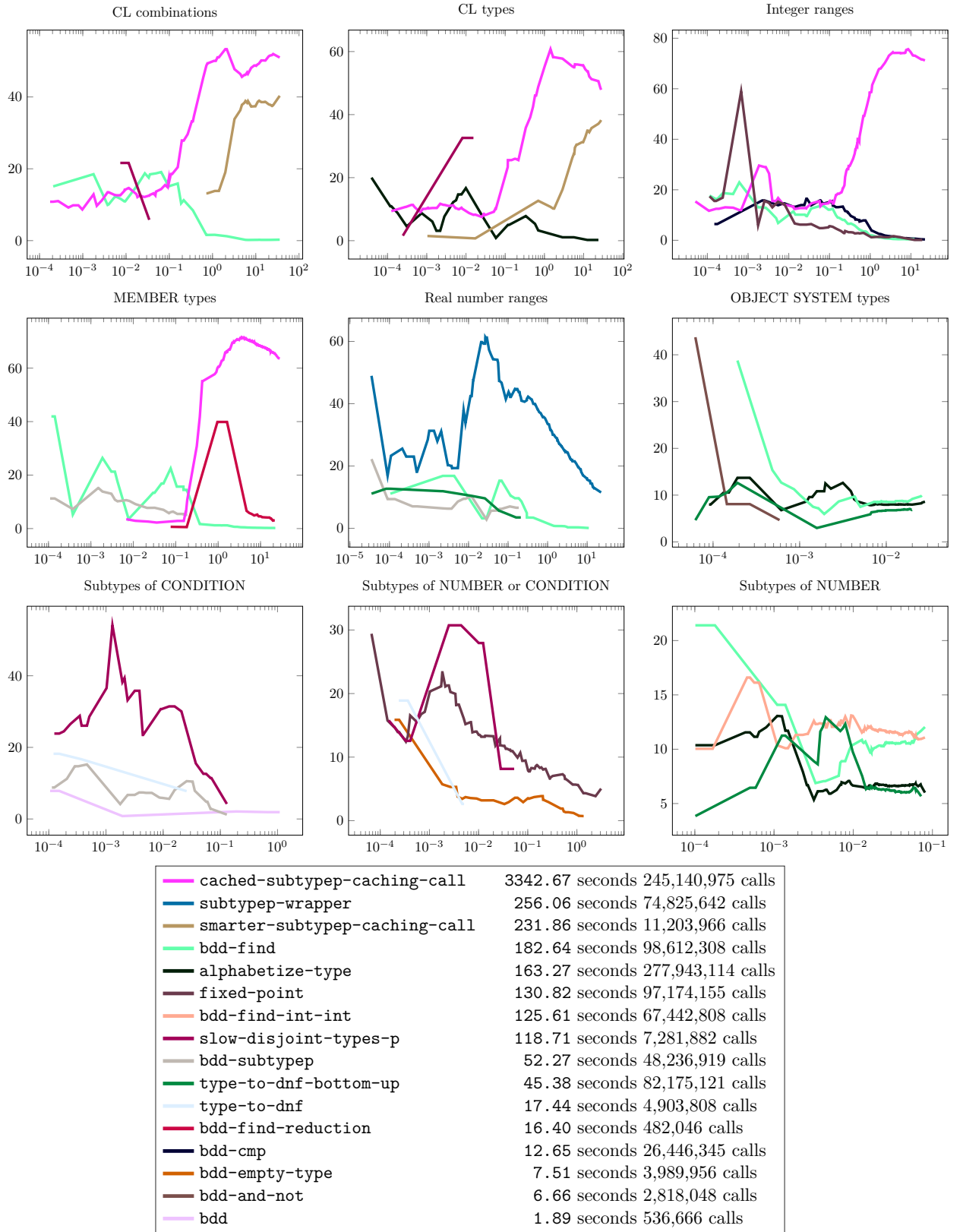
Figure 10.12: Performance Profile of various pools on algorithm mtd-bdd-weak-dynamic . Each plot is displayed with y ='Profile Percentage' vs. x ='Computation Time (seconds).'
