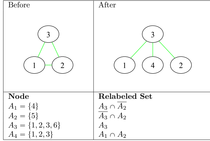
Figure 9.11: Connection between disjoint sets
