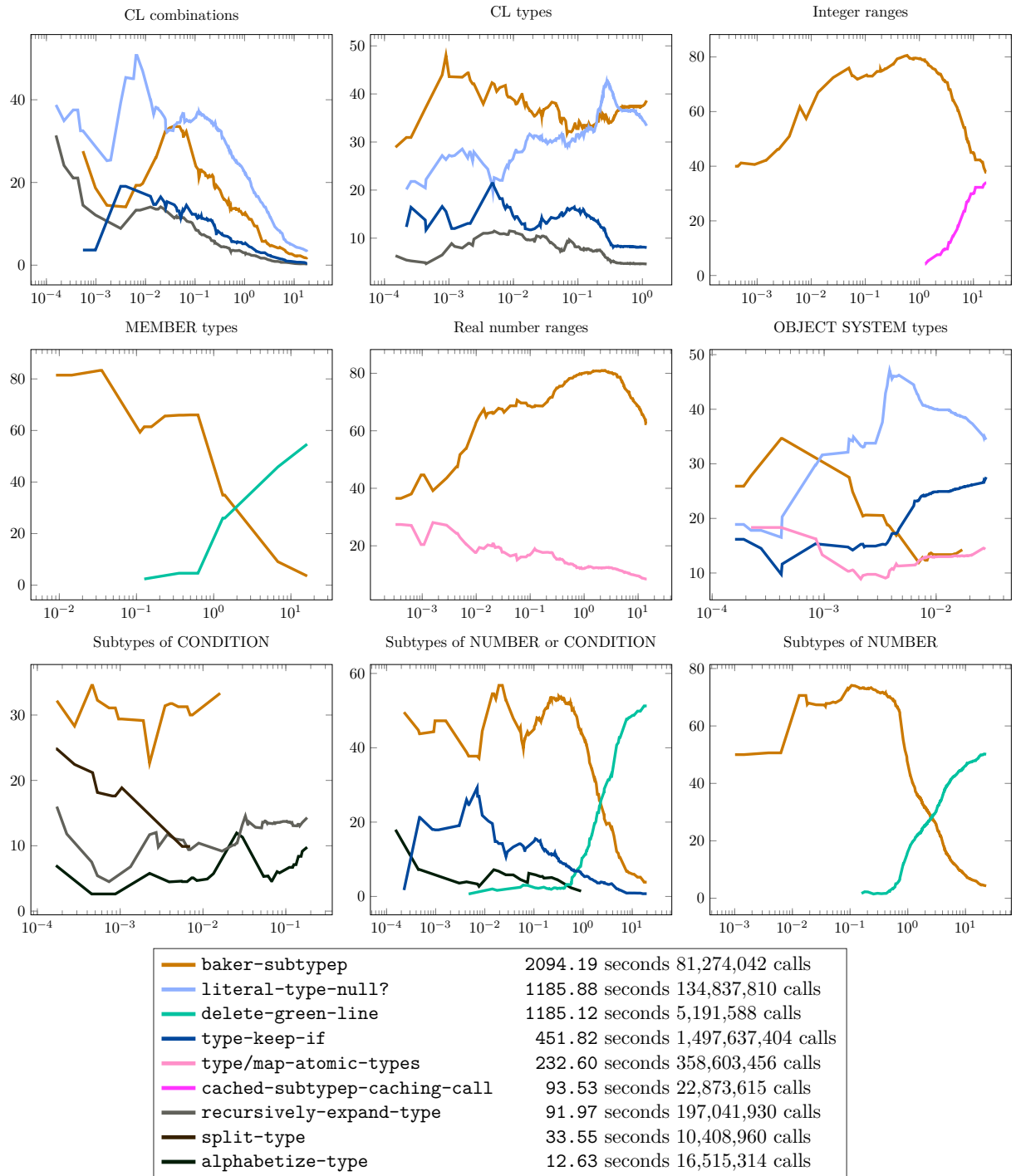
Figure 10.16: Performance Profile of various pools on algorithm mtd-graph-baker . Each plot is displayed with y='Profile Percentage' vs. x='Computation Time (seconds).'
