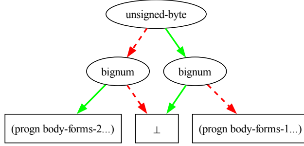
Figure 11.1: Decision Diagram representing irreducible typecase . This is similar to an ROBDD, but does not fulfill the definition thereof, because the leaf nodes are not simple Boolean values.
