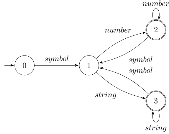
Figure 4.8: Example DFA implementing the rational type expression: (symbol \cdot (number^+ \cup string^+))^+
