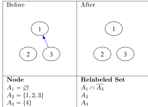
Figure 9.15: Connection between equal sets
