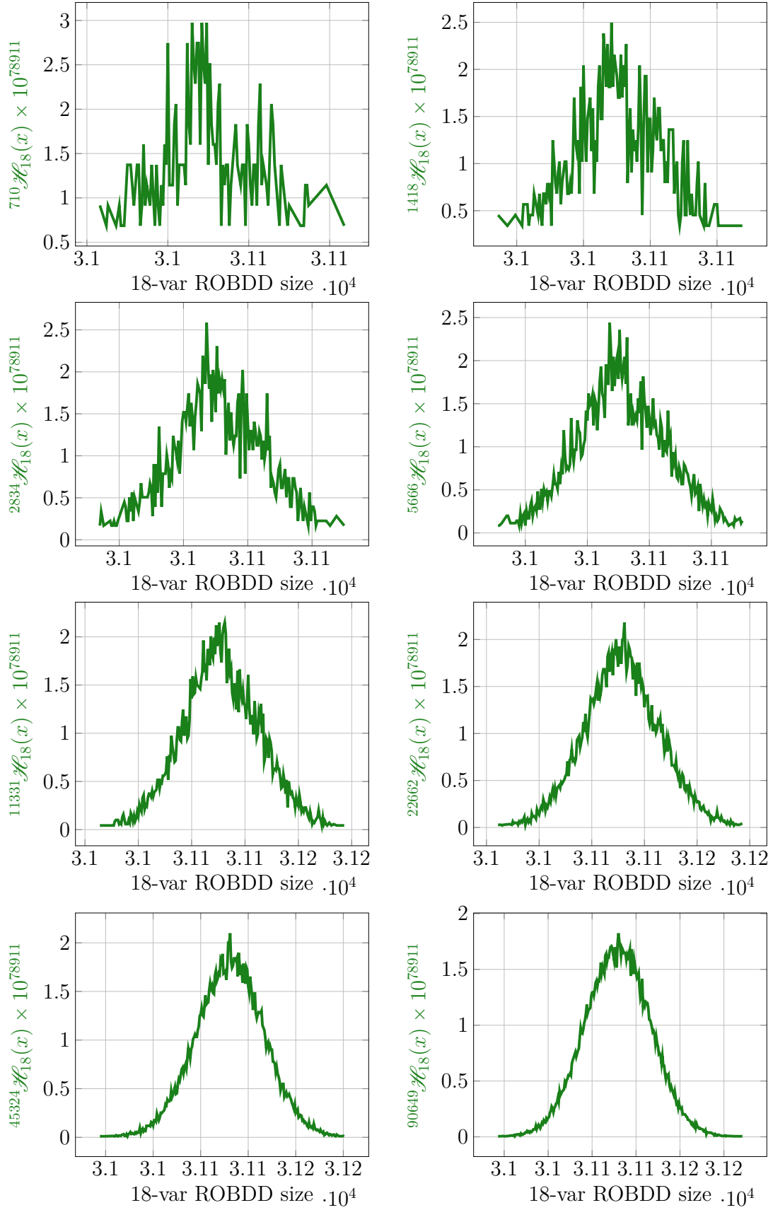
Figure 6.15: Histograms illustrating size distributions of successively larger samples for 18 variables. Each plot shows y = {}^M\mathcal{H}_{18} for successively larger values of M vs. x = \text{ROBDD size} .
