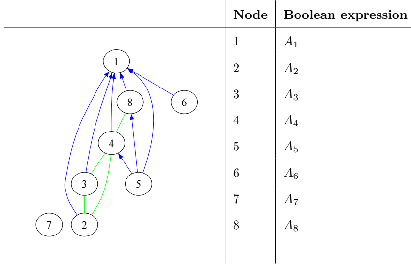
Figure 9.4: State 0: Topology graph
