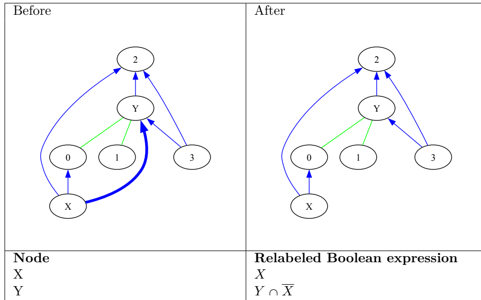
Figure 9.5: Strict subset before and after mutation
