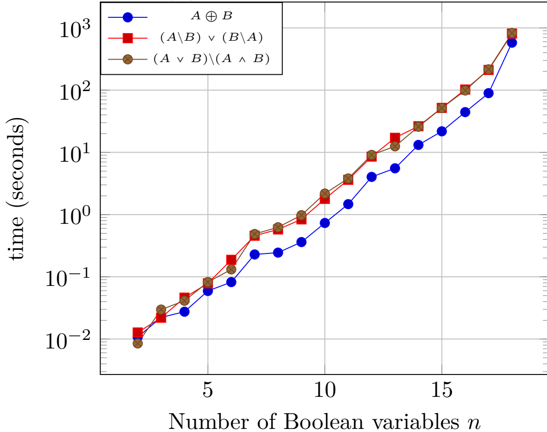
Figure 5.10: Comparison of execution time of three proposed implementations of the ROBDD xor, \oplus operator. The plot shows that calculating \oplus is usually faster using Equation (5.2) as opposed to Equation (5.4) or (5.5)
