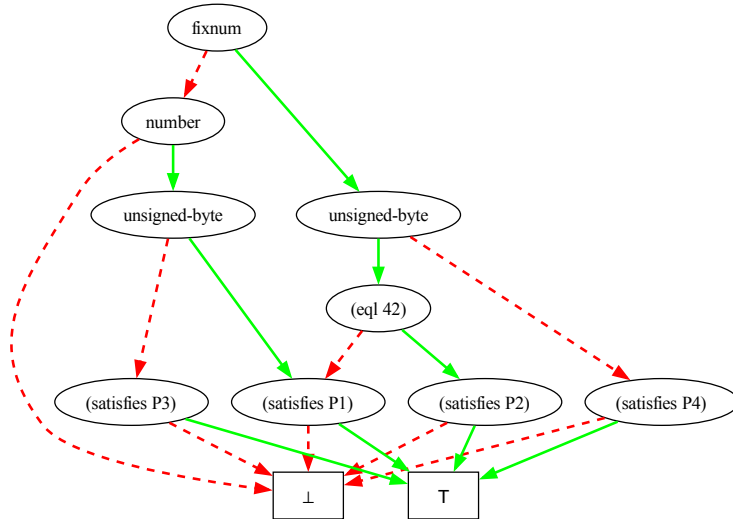
Figure 11.3: ROBDD generated from typecase clauses in Example 11.17
