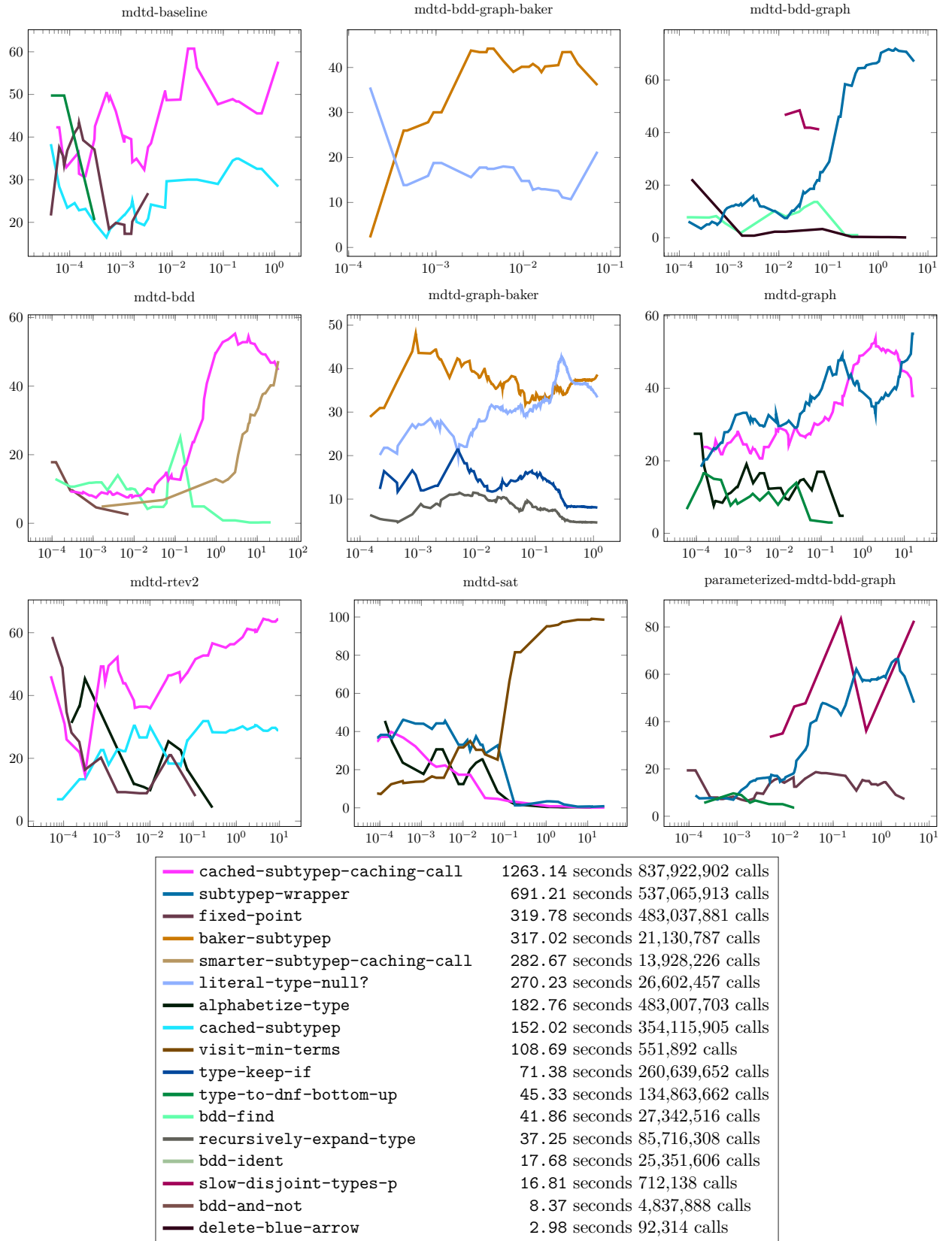
Figure 10.33: Performance Profile of various MDTD functions for pool CL types. Each plot is displayed with y = \text{'Profile Percentage'} vs. x = \text{'Computation Time (seconds)'} .
