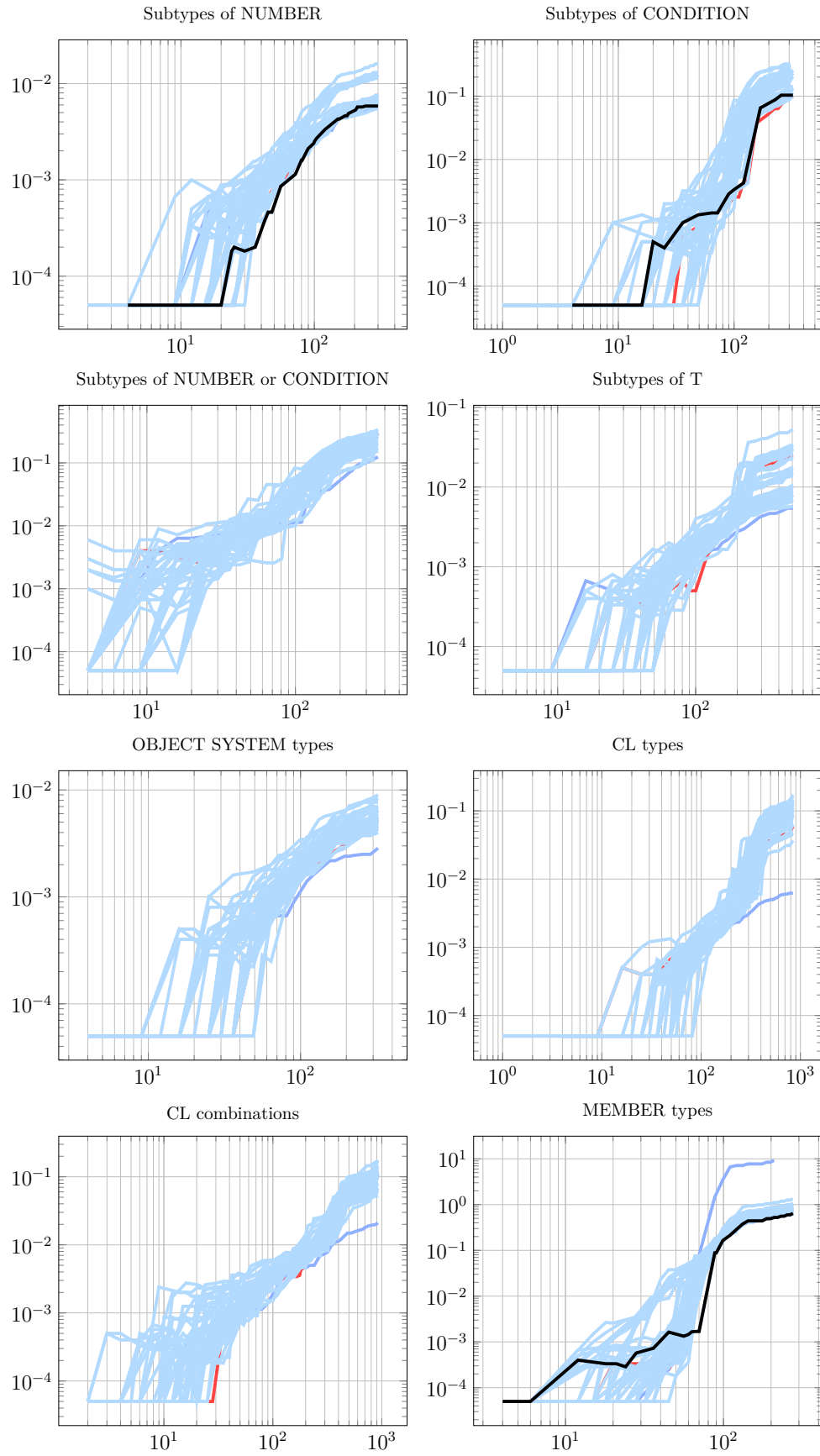
Figure 10.6: Tuning graph-based algorithm with various pools. Each plot is displayed with y ='Computation Time (seconds)' vs. x ='Product Size'.
