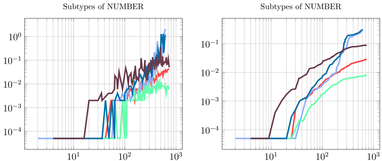
Figure 10.1: Run-time performance of MDTD algorithms applied to the pool consisting of subtypes of number. The plots show the measured data (left) and smoothed data (right). Each plot is displayed with y ='Computation Time (seconds)' vs. x ='Product Size'.
