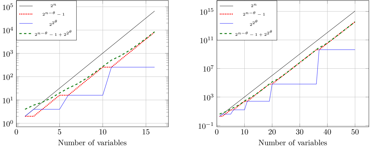
Figure 6.34: The plots show the relative sizes of 2^{n-\theta} , 2^{2\theta} , and their sum |ROBDD_n| .
