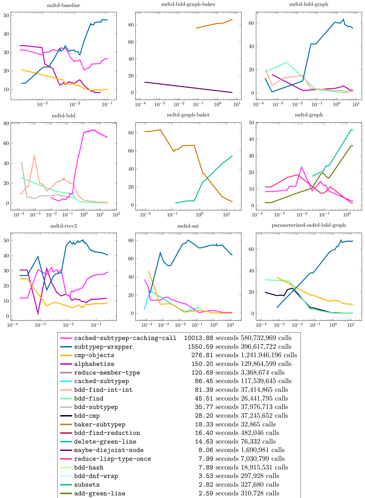
Figure 10.34: Performance Profile of various MDTD functions for pool MEMBER types. Each plot is displayed with y='Profile Percentage' vs. x='Computation Time (seconds).'
