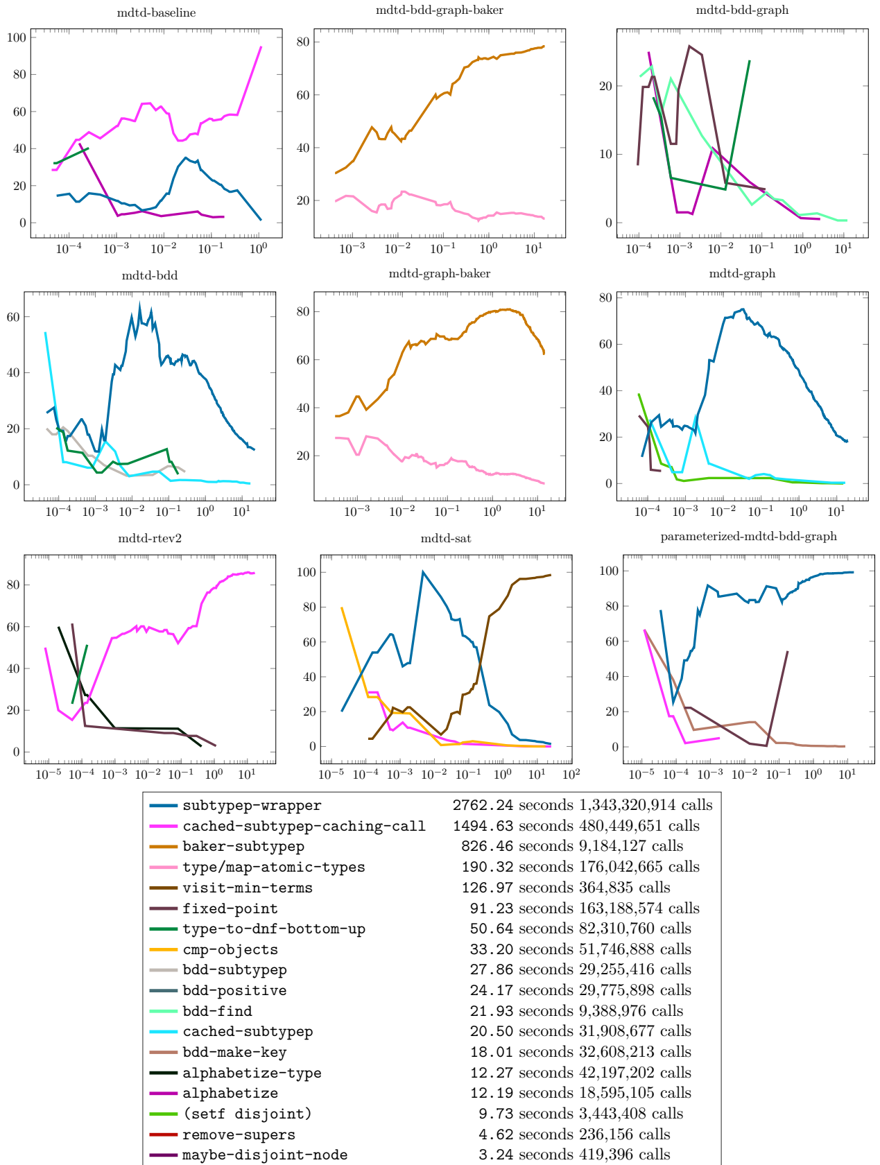
Figure 10.30: Performance Profile of various MDTD functions for pool Real number ranges . Each plot is displayed with y='Profile Percentage' vs. x='Computation Time (seconds).'
