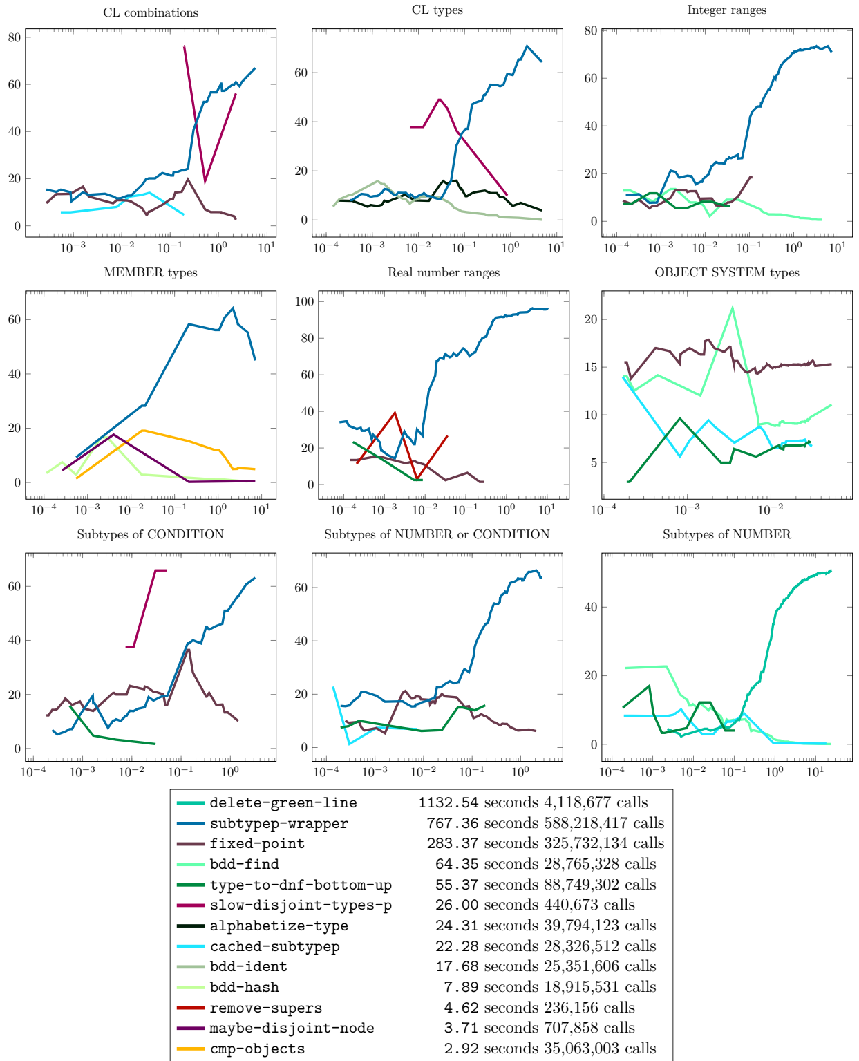
Figure 10.11: Performance Profile of various pools on algorithm mtd-bdd-graph-weak-dynamic . Each plot is displayed with y='Profile Percentage' vs. x='Computation Time (seconds).'
