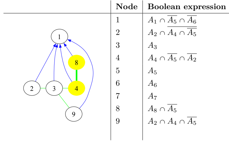
Figure F.3: State 2: Topology graph after disconnecting 2 from 4
