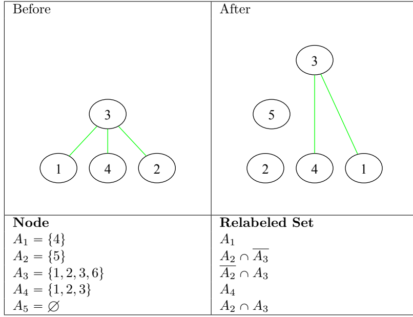
Figure 9.12: Discovered Empty Set
