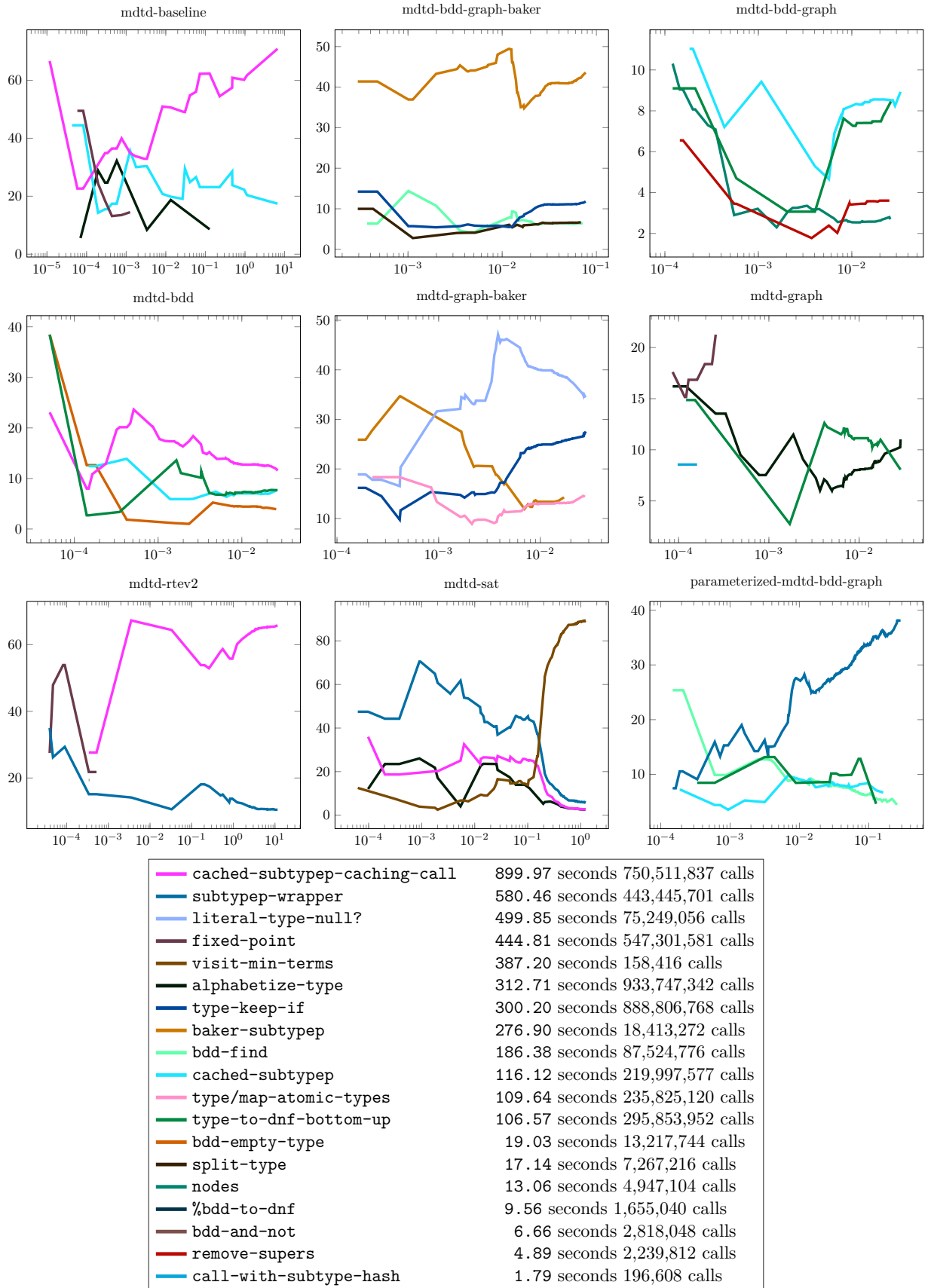
Figure 10.32: Performance Profile of various MDTD functions for pool OBJECT SYSTEM types. Each plot is displayed with y='Profile Percentage' vs. x='Computation Time (seconds)'.
