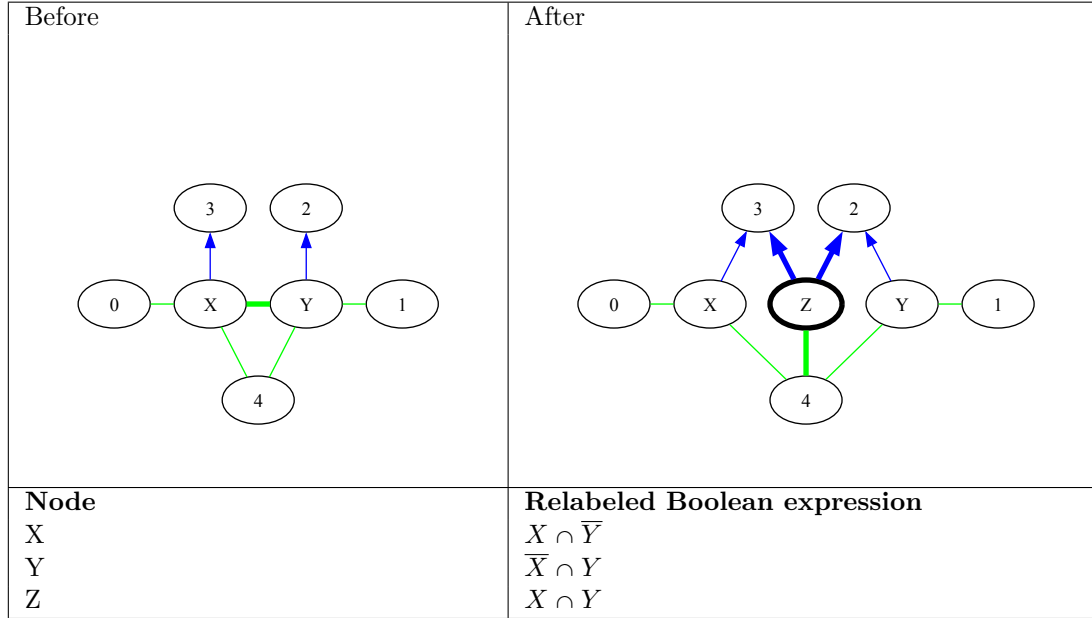
Figure 9.8: Touching connections before and after mutation
