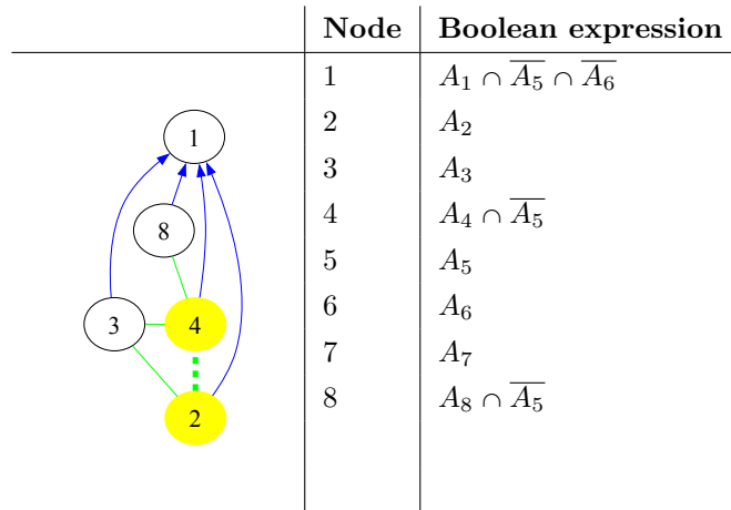
Figure F.2: State 1: Topology graph, after isolating 5 and 6.
