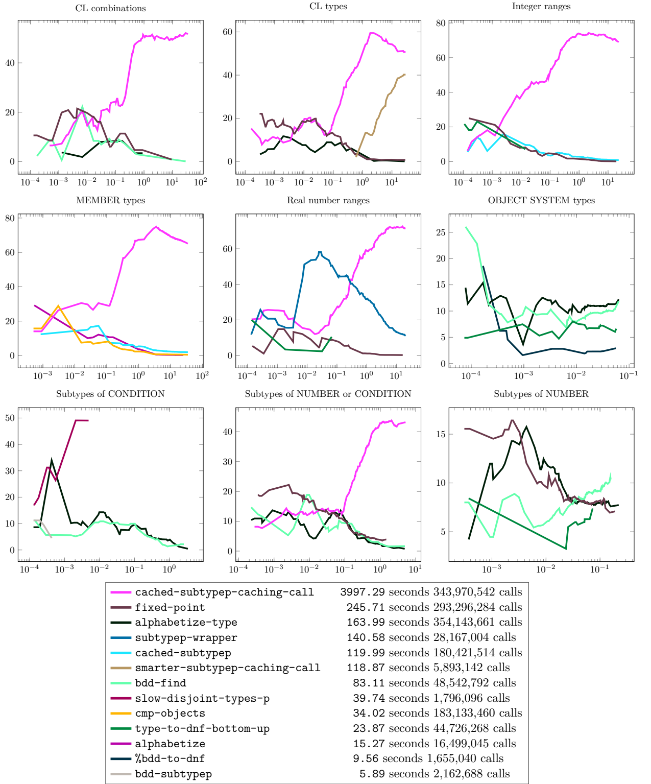
Figure 10.20: Performance Profile of various pools on algorithm mtd-bdd-weak . Each plot is displayed with y = \text{'Profile Percentage'} vs. x = \text{'Computation Time (seconds)'} .
