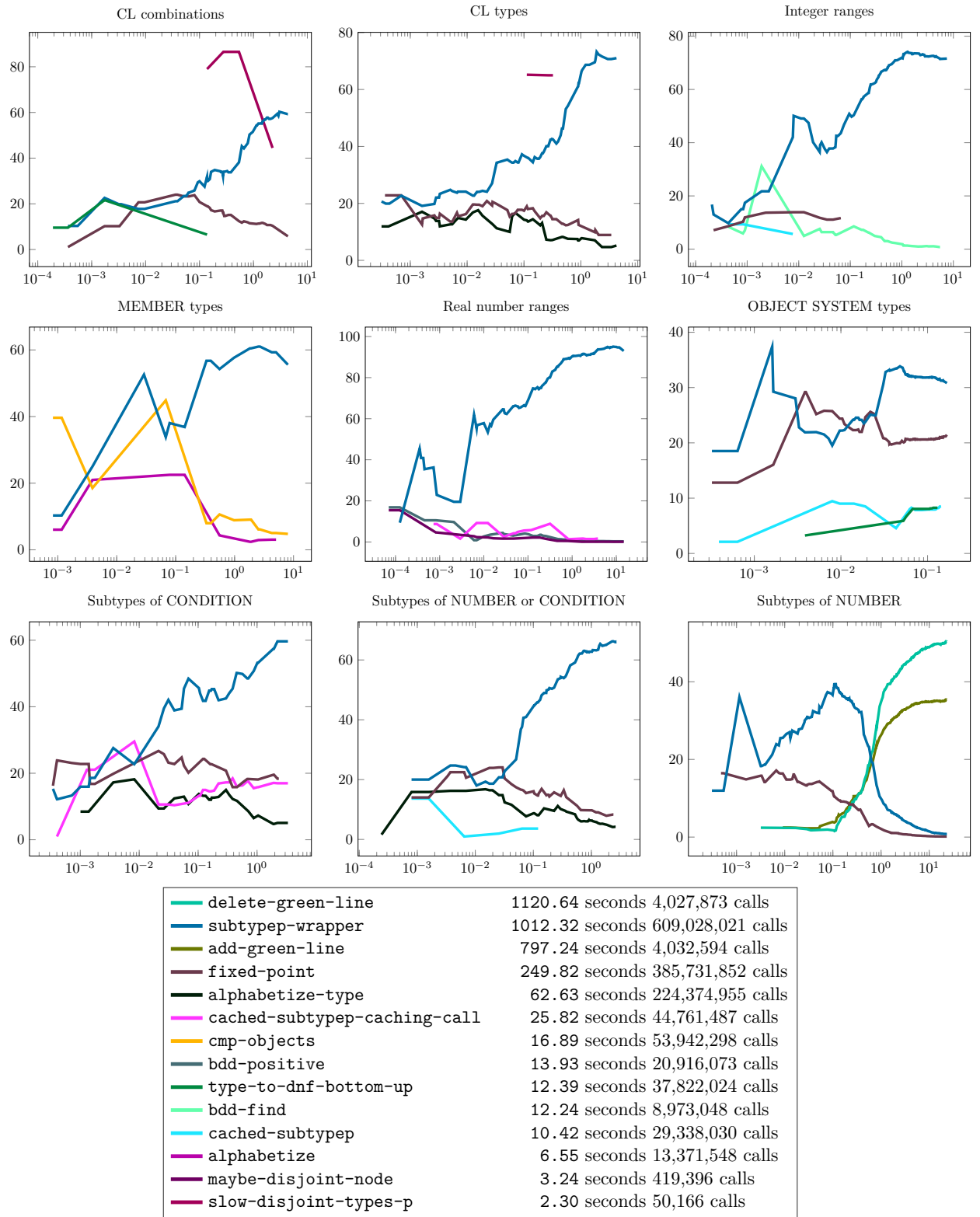
Figure 10.13: Performance Profile of various pools on algorithm mtd-bdd-graph-strong . Each plot is displayed with y =‘Profile Percentage’ vs. x =‘Computation Time (seconds)’.
