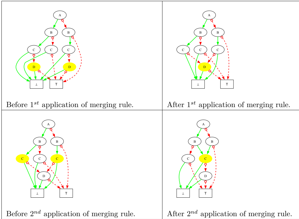
Figure 5.7: Examples of Merging Rule. The highlighted nodes in the left hand-column are congruent. One is deleted, one remains, as shown in the right-hand column.
