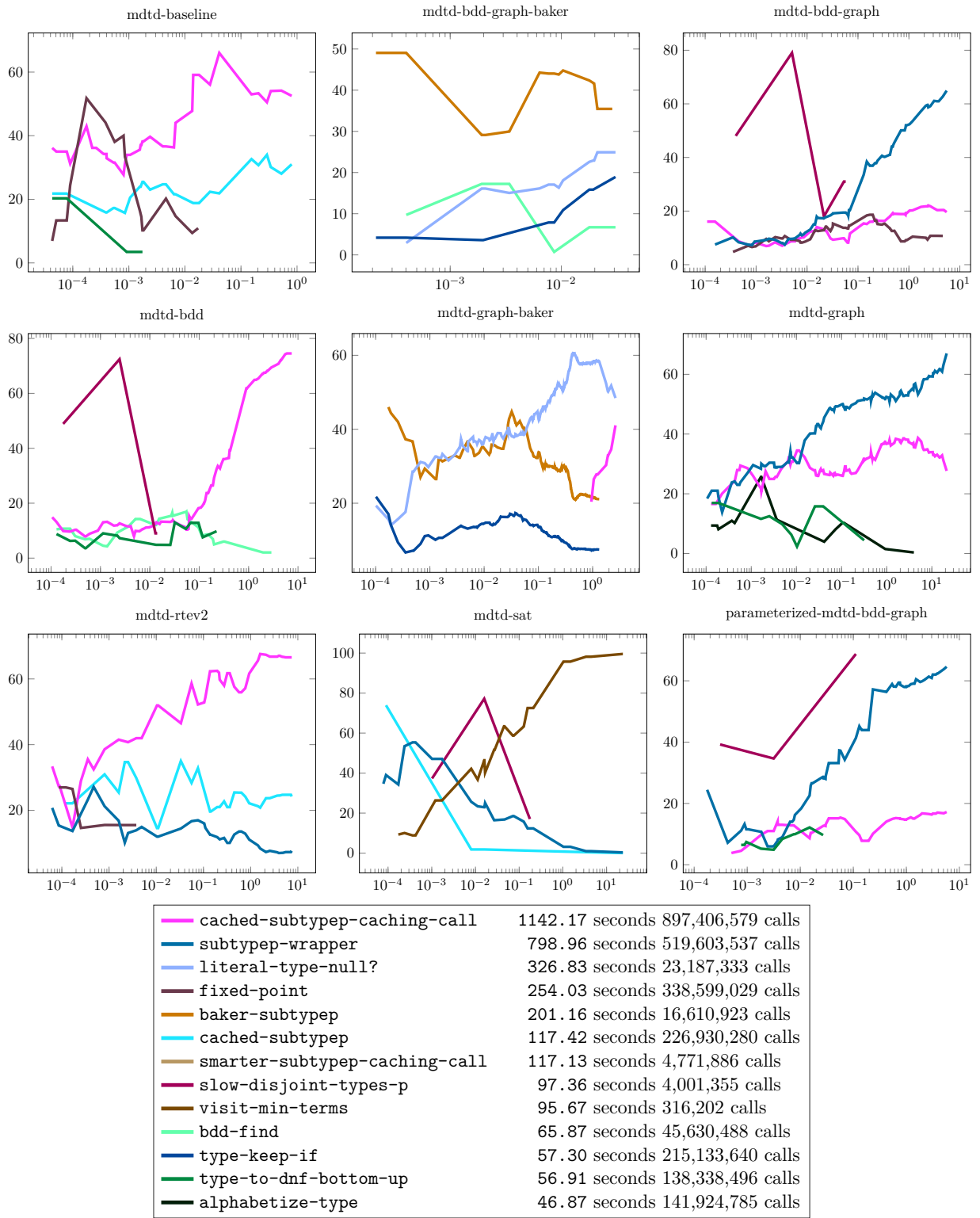
Figure 10.29: Performance Profile of various MDTD functions for pool Subtypes of T . Each plot is displayed with y='Profile Percentage' vs. x='Computation Time (seconds).'
