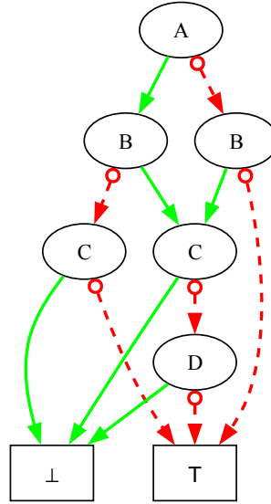
Figure 5.5: BDD after applying Terminal, Deletion, and Merging rules. This diagram is an ROBDD logically equivalent to the UOBDD shown in Figure 5.2.
