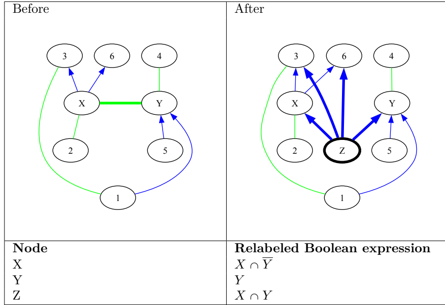
Figure 9.9: Graph meeting the loop condition
