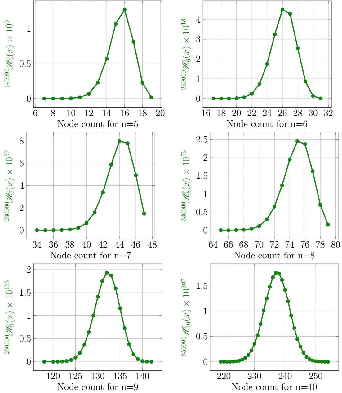
Figure 6.4: Histograms illustrating size distributions of ROBDDs from 5 to 10. The histograms are based on extrapolations from sampled data. The plots show y = M \mathcal{H}_n vs x = \text{ROBDD size} , for 5 \leq n \leq 10 , and in each case with the maximum value of M from our experiments.
