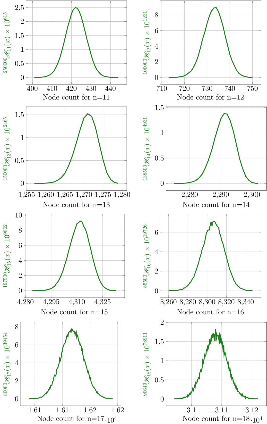
Figure 6.5: Histograms illustrating size distributions of ROBDDs from 11 to 18. The histograms are based on extrapolations from sampled data. The plots show y = {}^M\mathcal{H}_n vs x = \text{ROBDD size} , for 11 \leq n \leq 18 , and in each case with the maximum value of M from our experiments.
