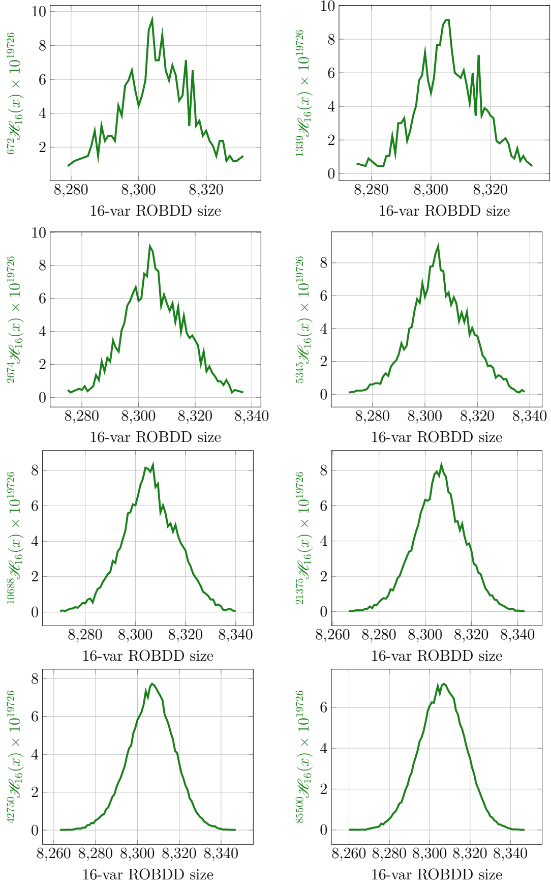
Figure 6.14: Histograms illustrating size distributions of successively larger samples for 16 variables. Each plot shows y = {}^M\mathcal{H}_{16} for successively larger values of M vs. x = \text{ROBDD size} .
