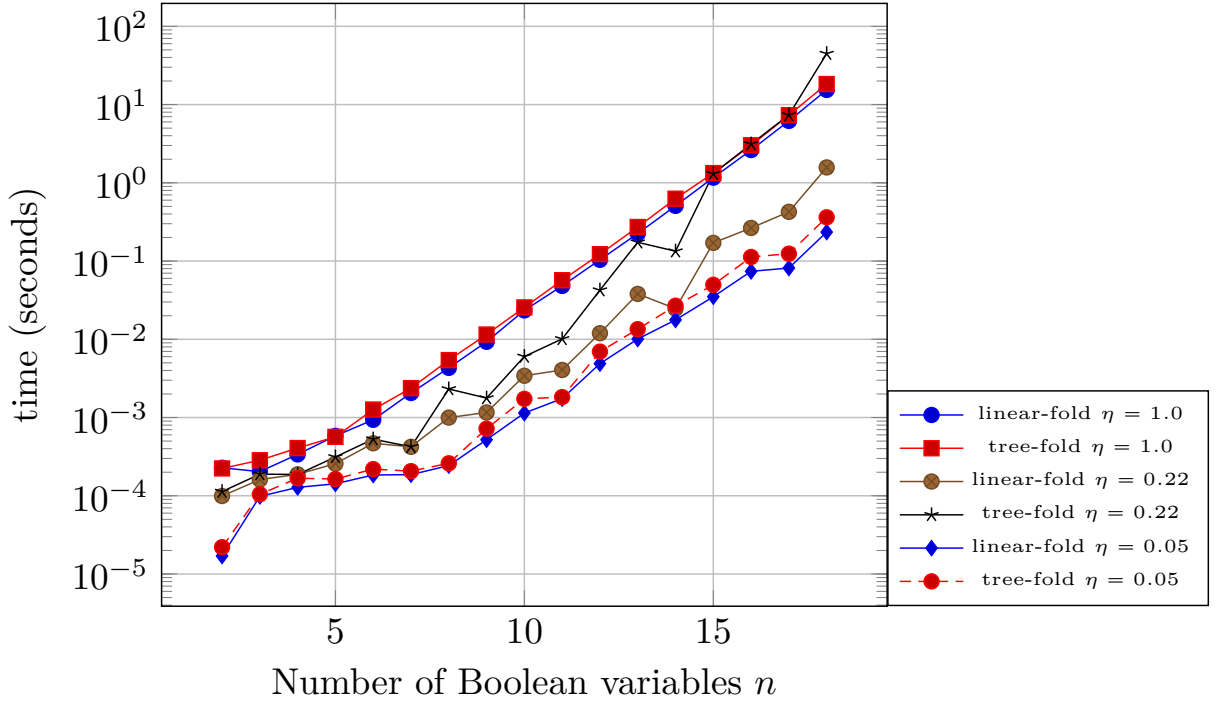
Figure 5.11: Comparison of ROBDD construction time using linear and tree-like fold operations. The times are plotted for various values of \eta .
