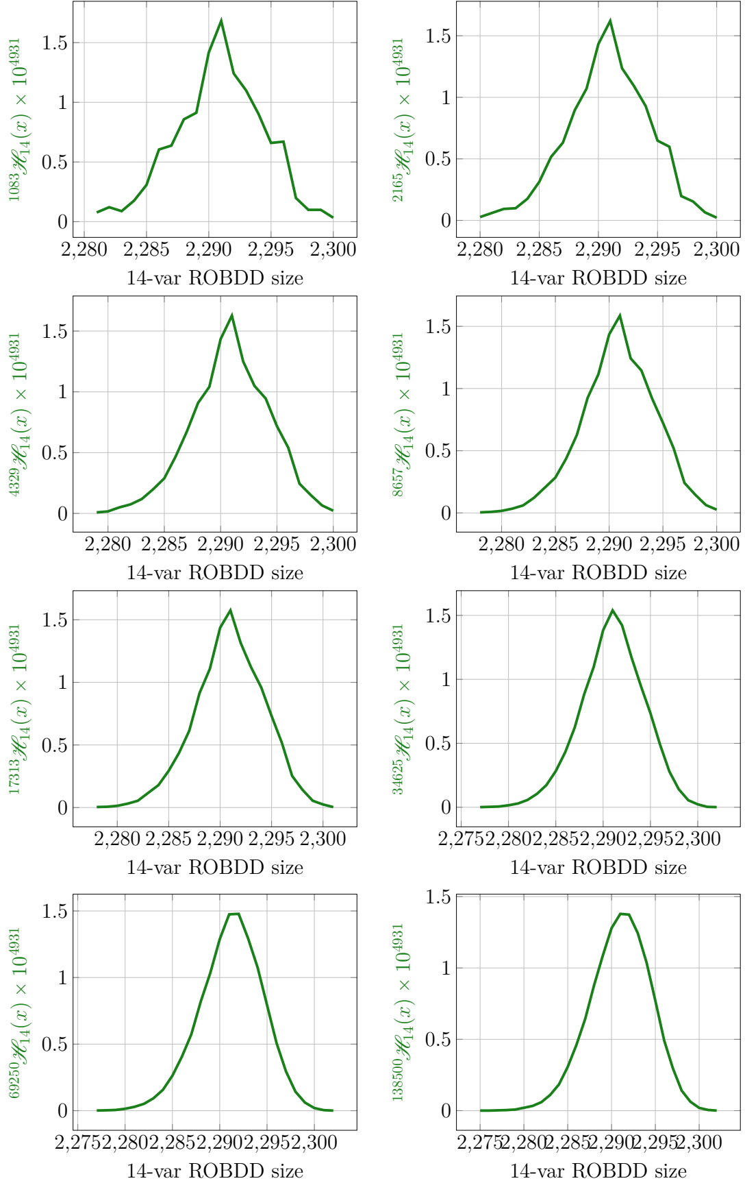
Figure 6.13: Histograms illustrating size distributions of successively larger samples for 14 variables. Each plot shows y = {}^M \mathcal{H}_{14} for successively larger values of M vs. x = \text{ROBDD size} .
