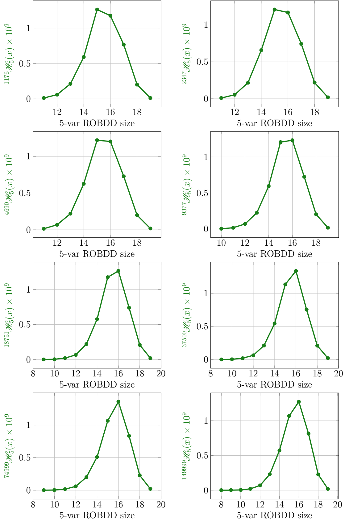
Figure 6.10: Histograms illustrating size distributions of successively larger samples for 5 variables. Each plot shows y = M \mathcal{H}_5 for successively larger values of M vs. x = \text{ROBDD size} .
