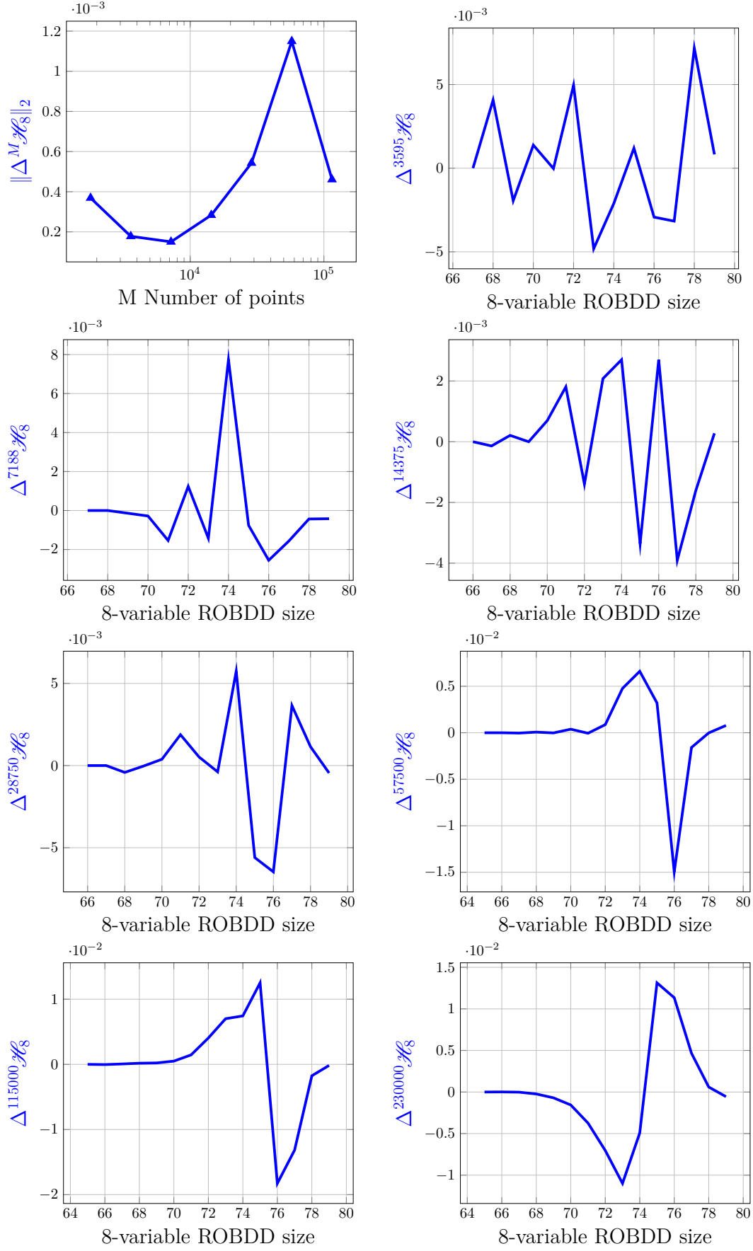
Figure 6.24: Difference functions for n = 8
