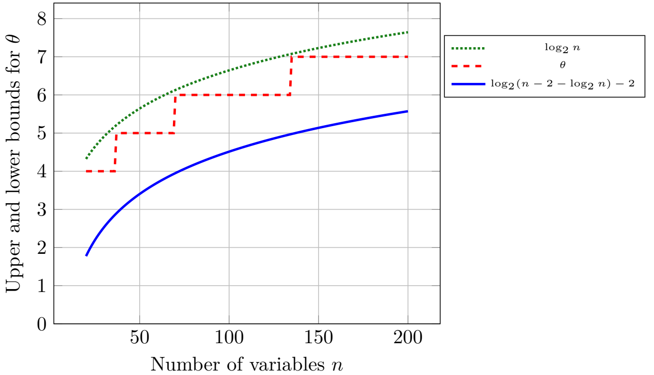
Figure 6.32: Upper and lower bounds for \theta
