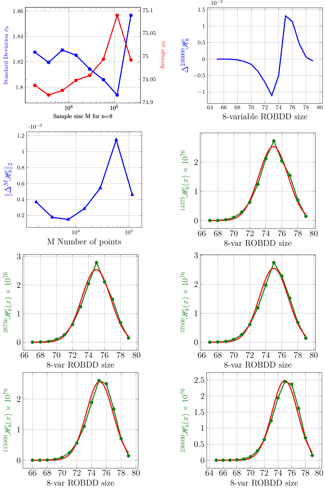
Figure 6.19: Histograms (from Figure 6.11) illustrating size distributions of successively larger samples for 8 variables, shown along with the theoretical normal distribution having the same \mu_8 and \sigma_8 . This figure also shows (top left) the plots of y = \mu_8 and y = \sigma_8 vs. x = node count for successively larger values of M . The plot in top right shows the difference function y = \Delta^M \mathcal{H}_8 for the maximum sample size taken, M . Also shown in the plot of y = \|\Delta^M \mathcal{H}_8\|_2 for successively larger values of M which serves as an indicator of convergence of the \mathcal{H}_8 curves.
