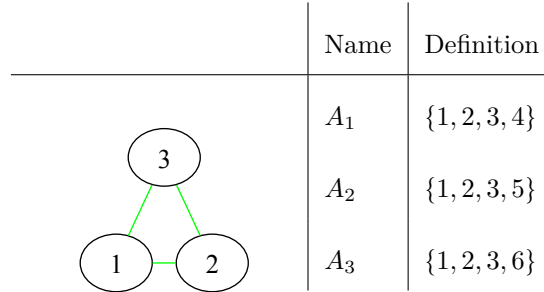
Figure 9.10: Setup for Discovered Empty Set
