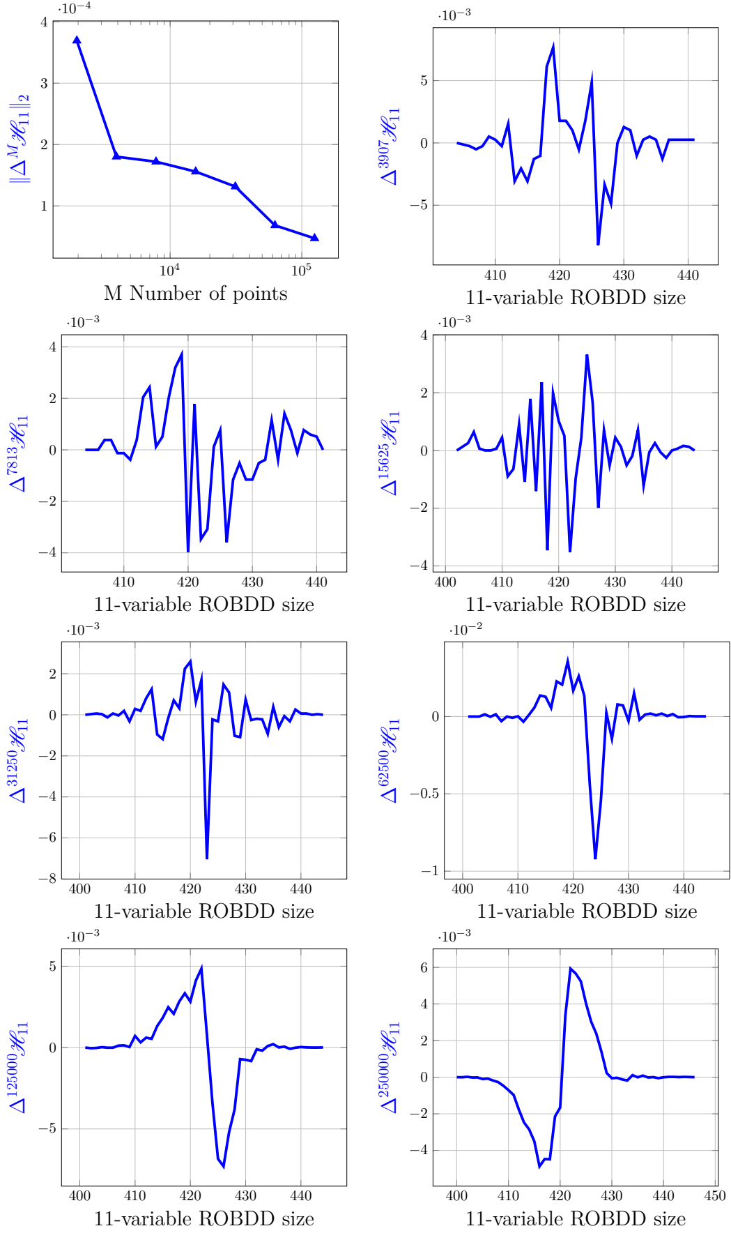
Figure 6.25: Difference functions for n = 11
