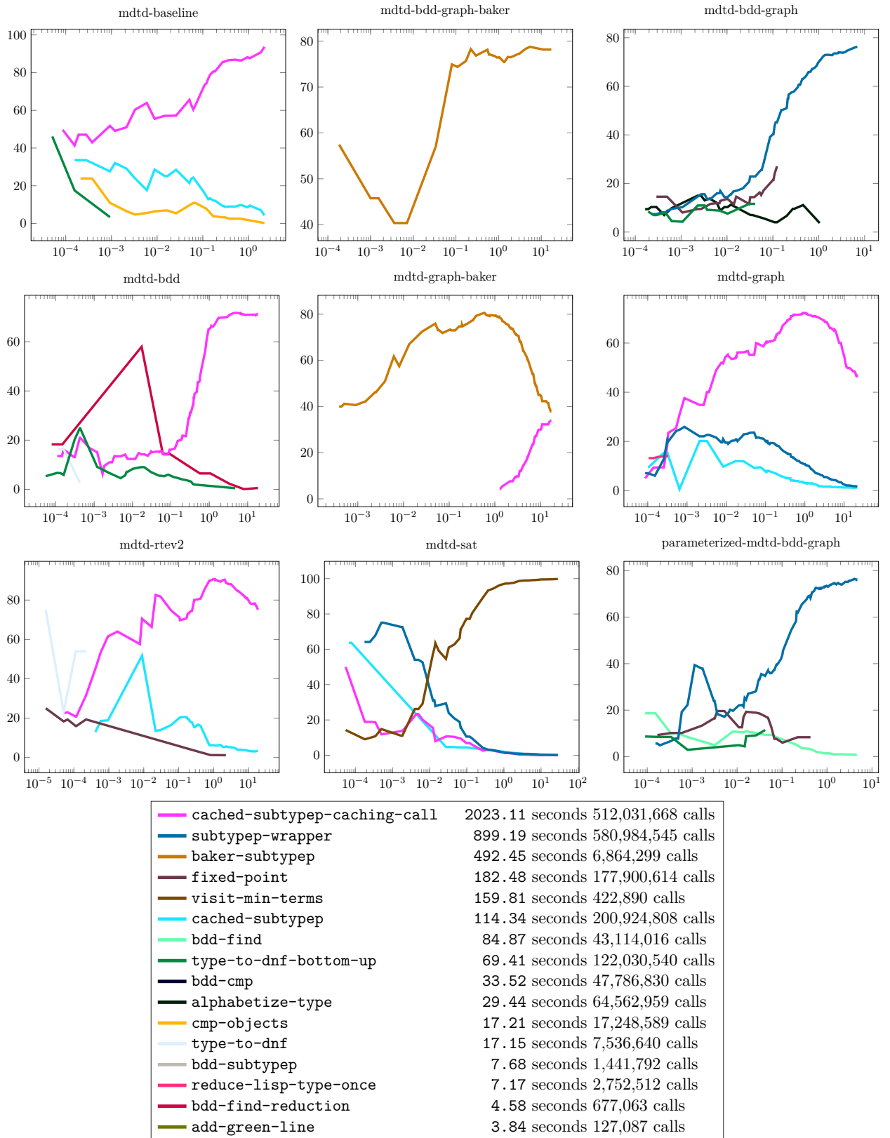
Figure 10.28: Performance Profile of various MDTD functions for pool Integer ranges. Each plot is displayed with y='Profile Percentage' vs. x='Computation Time (seconds).'
