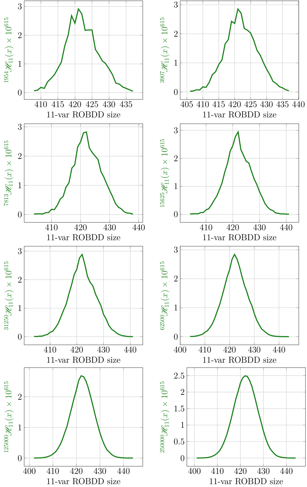
Figure 6.12: Histograms illustrating size distributions of successively larger samples for 11 variables. Each plot shows y = {}^M\mathcal{H}_{11} for successively larger values of M vs. x = \text{ROBDD size} .
