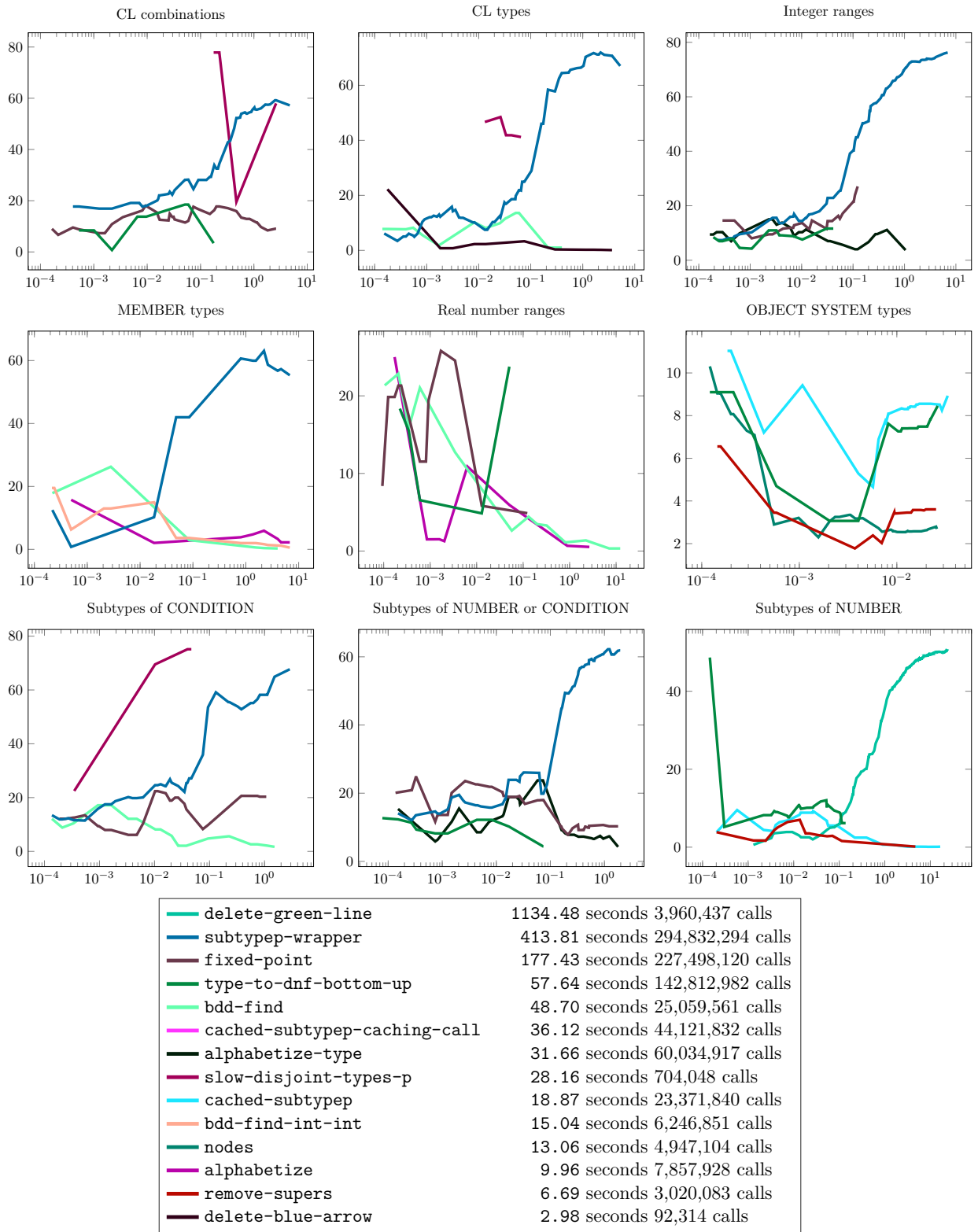
Figure 10.18: Performance Profile of various pools on algorithm mtd-bdd-graph . Each plot is displayed with y ='Profile Percentage' vs. x ='Computation Time (seconds).'
