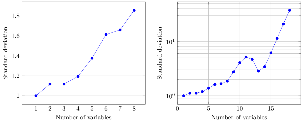
Figure 6.9: Standard deviations for each of the curves shown in Figure 6.7 and whose averages are shown in Figure 6.8.
