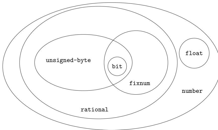
Figure 2.1: Some example Common Lisp types showing their intersection and subset relations
