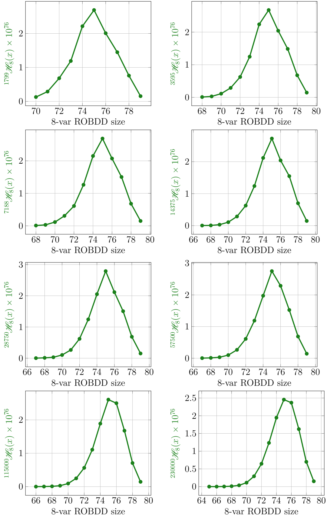
Figure 6.11: Histograms illustrating size distributions of successively larger samples for 8 variables. Each plot shows y = M \mathcal{H}_8 for successively larger values of M vs. x = \text{ROBDD size} .
