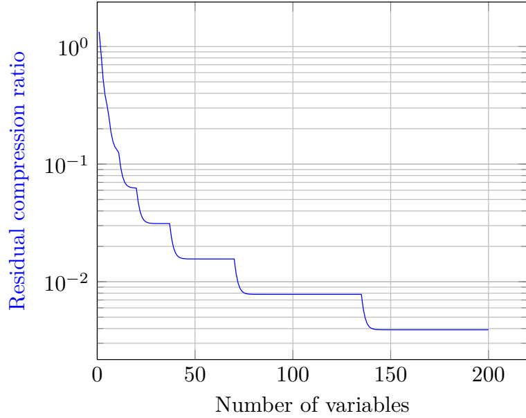
Figure 6.35: Residual compression ratio of worst-case ROBDD, calculated from theoretical data as compared to UOBDD, and shown in tabular graphical form.
