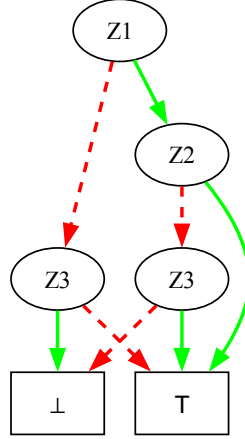
Figure 5.1: BDD for (Z_1 \wedge Z_2) \vee (Z_1 \wedge \neg Z_2 \wedge Z_3) \vee (\neg Z_1 \wedge \neg Z_3)
