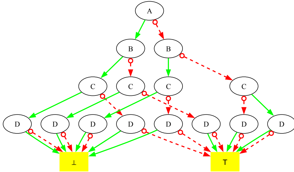
Figure 5.4: BDD after applying Terminal rule
