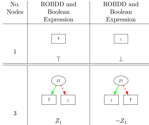
Figure 6.1: All ROBDDs of one variable
