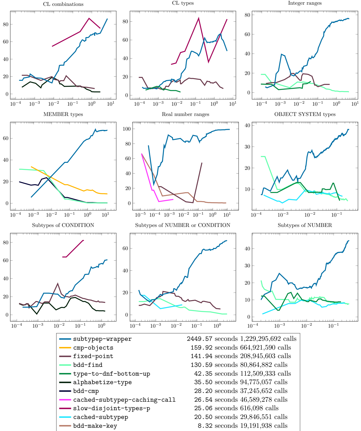
Figure 10.10: Performance Profile of various pools on algorithm parameterized-mdtd-bdd-graph . Each plot is displayed with y = \text{'Profile Percentage'} vs. x = \text{'Computation Time (seconds)'} .
