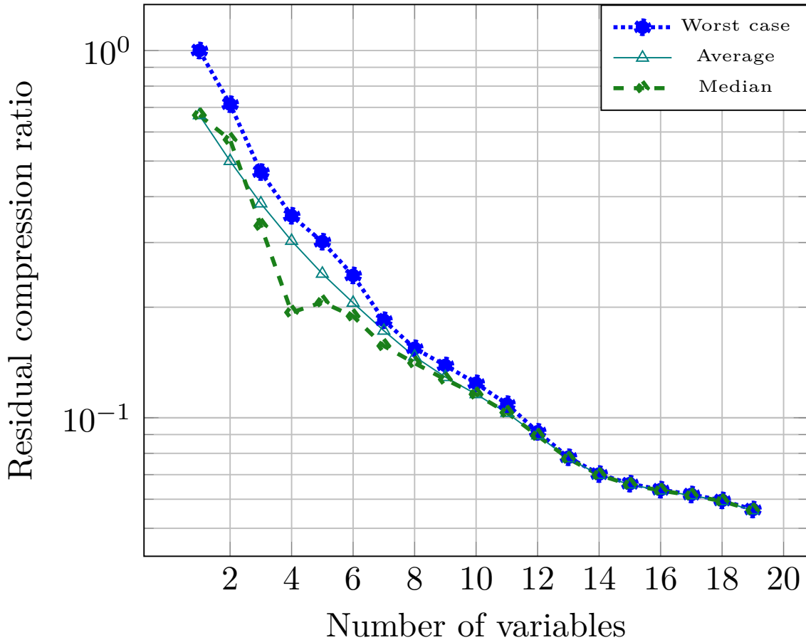
Figure 6.28: Residual compression ratio of ROBDD as compared to UOBDD
