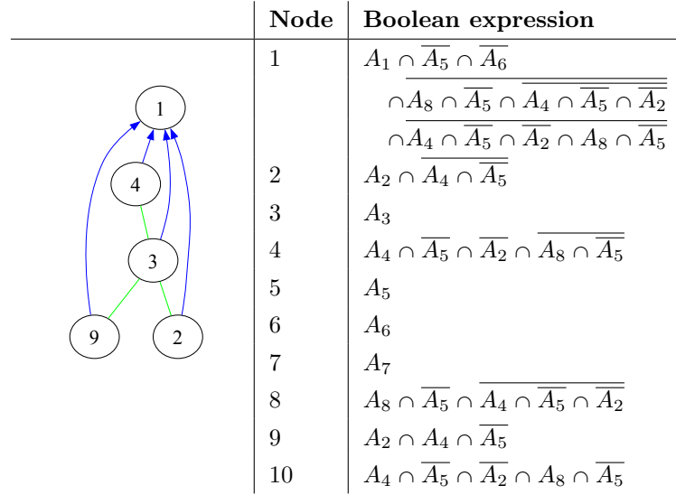
Figure F.5: State 4: Topology graph after isolating 8 and 10
