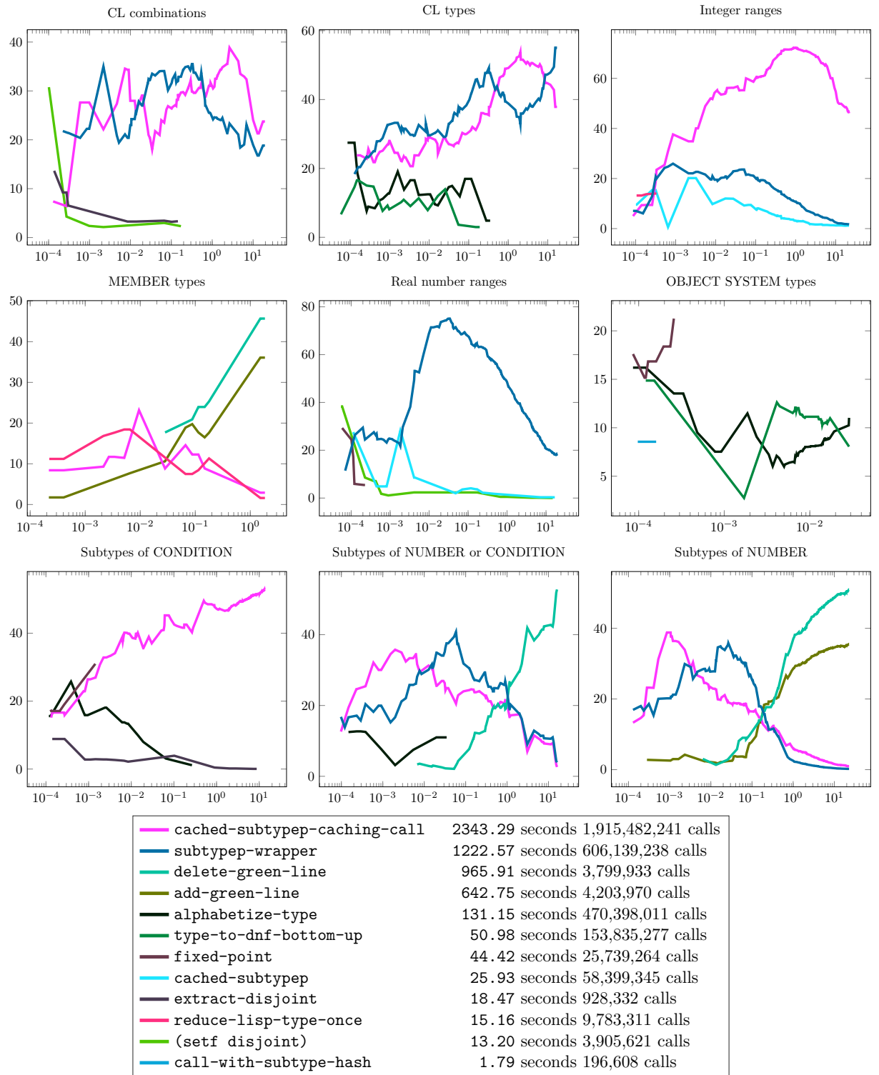
Figure 10.22: Performance Profile of various pools on algorithm mdtd-graph . Each plot is displayed with y ='Profile Percentage' vs. x ='Computation Time (seconds).'
