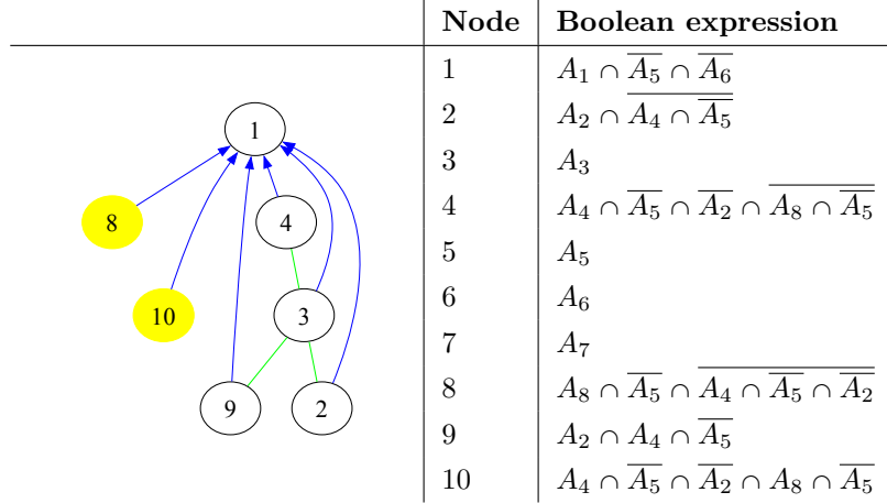
Figure F.4: State 3: Topology graph after disconnecting 4 from 8
