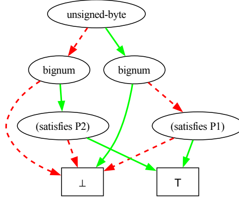
Figure 11.2: ROBDD with temporary valid satisfies types
