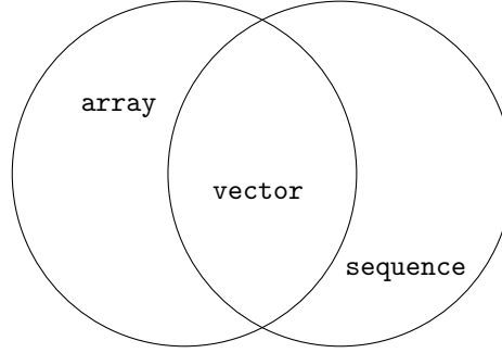
Figure 9.3: Relation of vector , sequence , and array . vector is identically the intersection of array and sequence .
