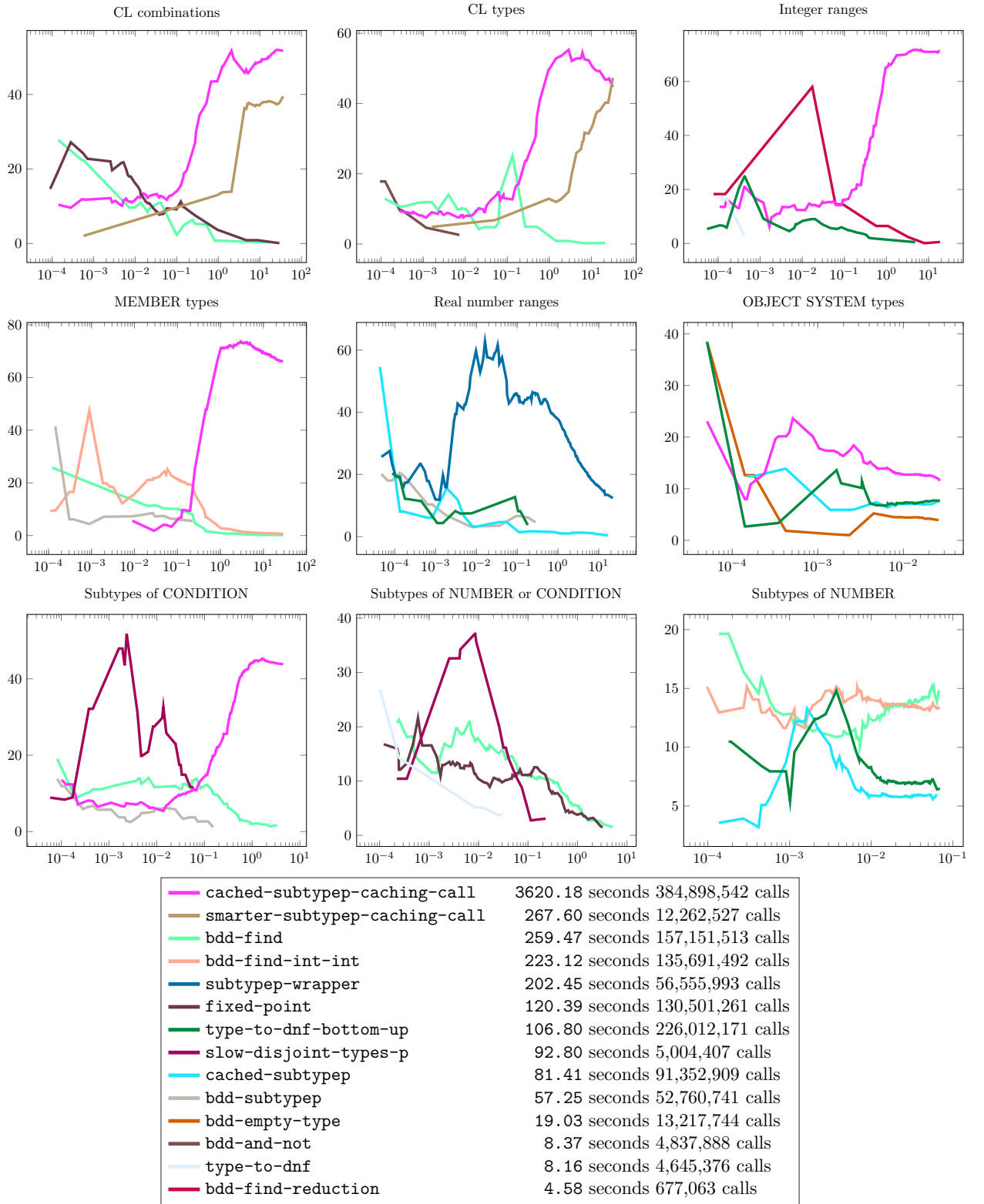
Figure 10.24: Performance Profile of various pools on algorithm mtd-bdd . Each plot is displayed with y ='Profile Percentage' vs. x ='Computation Time (seconds).'
