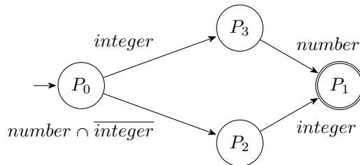
Figure 4.10: Example DFA with disjoint types
