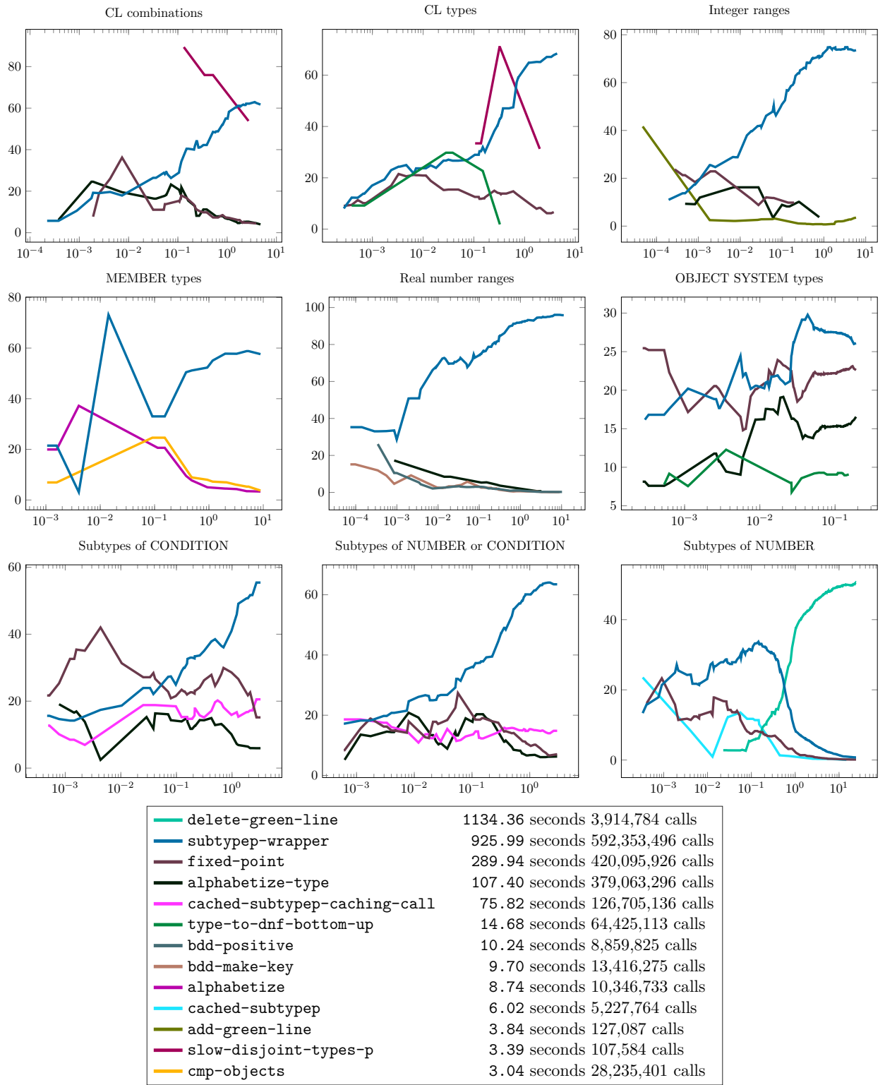
Figure 10.15: Performance Profile of various pools on algorithm mtdt-bdd-graph-weak . Each plot is displayed with y = \text{'Profile Percentage'} vs. x = \text{'Computation Time (seconds)'} .
