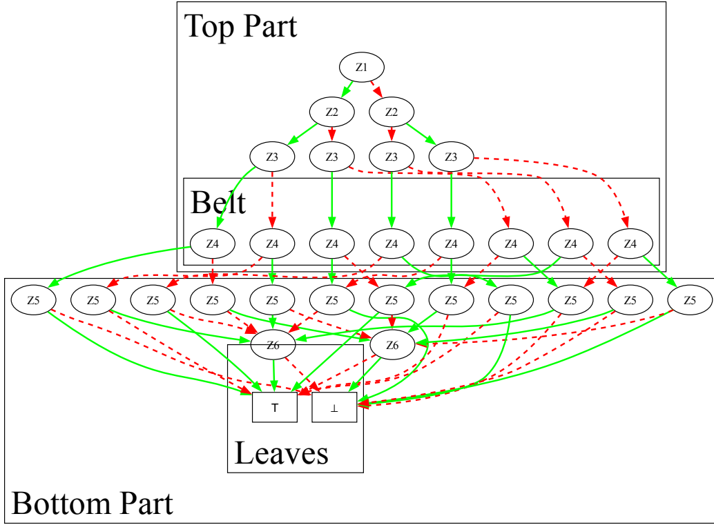
Figure 6.30: Example shape of a worst-case ROBDD. This figure shows 6-variable ROBDD with top & bottom parts marked. The figure also highlights the belt and leaves. Section 6.2 explains the construction of this ROBDD. In particular the leaves, bottom part, belt and top part are specifically constructed in Algorithms 4 and 5. The formula for the row index of the belt is given in Equation (6.29)
