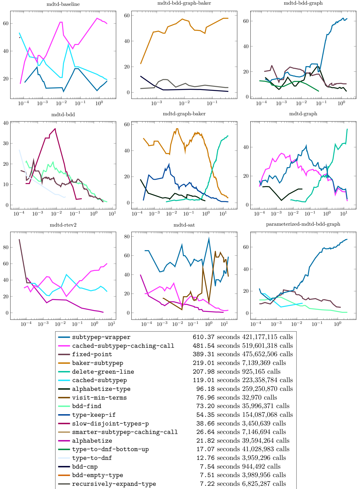
Figure 10.25: Performance Profile of various MDTD functions for pool Subtypes of NUMBER or CONDITION . Each plot is displayed with y='Profile Percentage' vs. x='Computation Time (seconds).'
