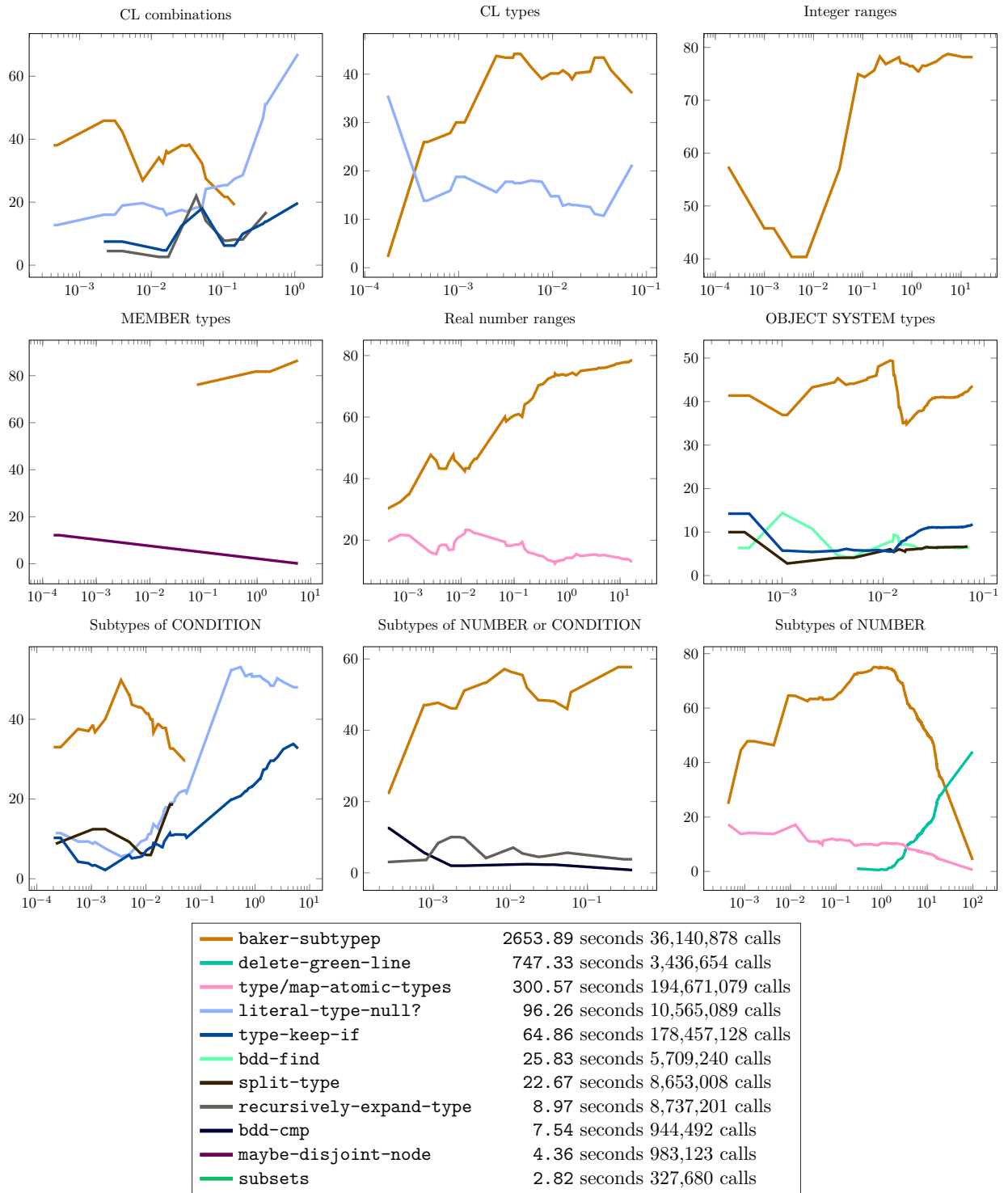
Figure 10.14: Performance Profile of various pools on algorithm mtd-bdd-graph-baker . Each plot is displayed with y = \text{'Profile Percentage'} vs. x = \text{'Computation Time (seconds)'} .
