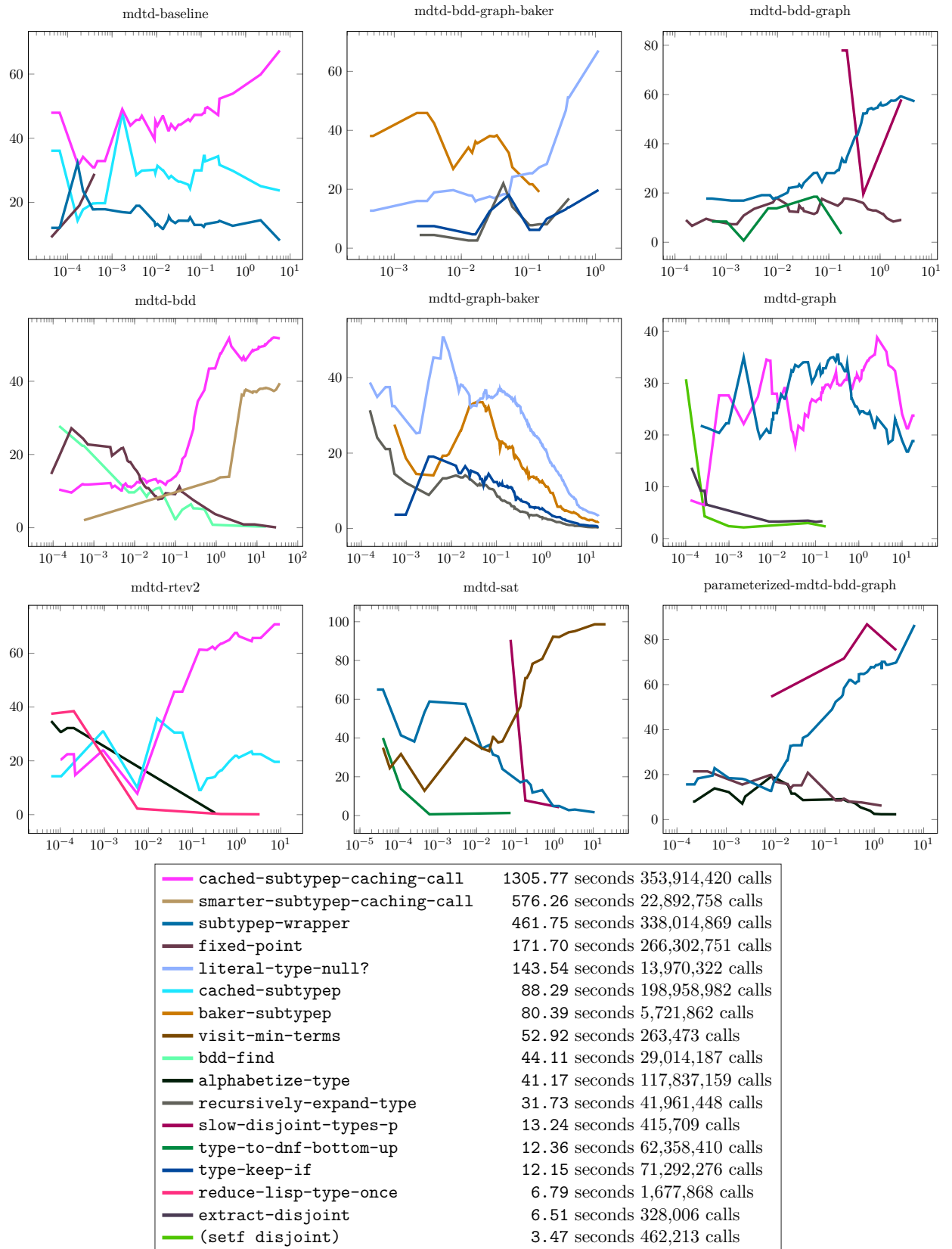
Figure 10.31: Performance Profile of various MDTD functions for pool CL combinations . Each plot is displayed with y='Profile Percentage' vs. x='Computation Time (seconds).'
