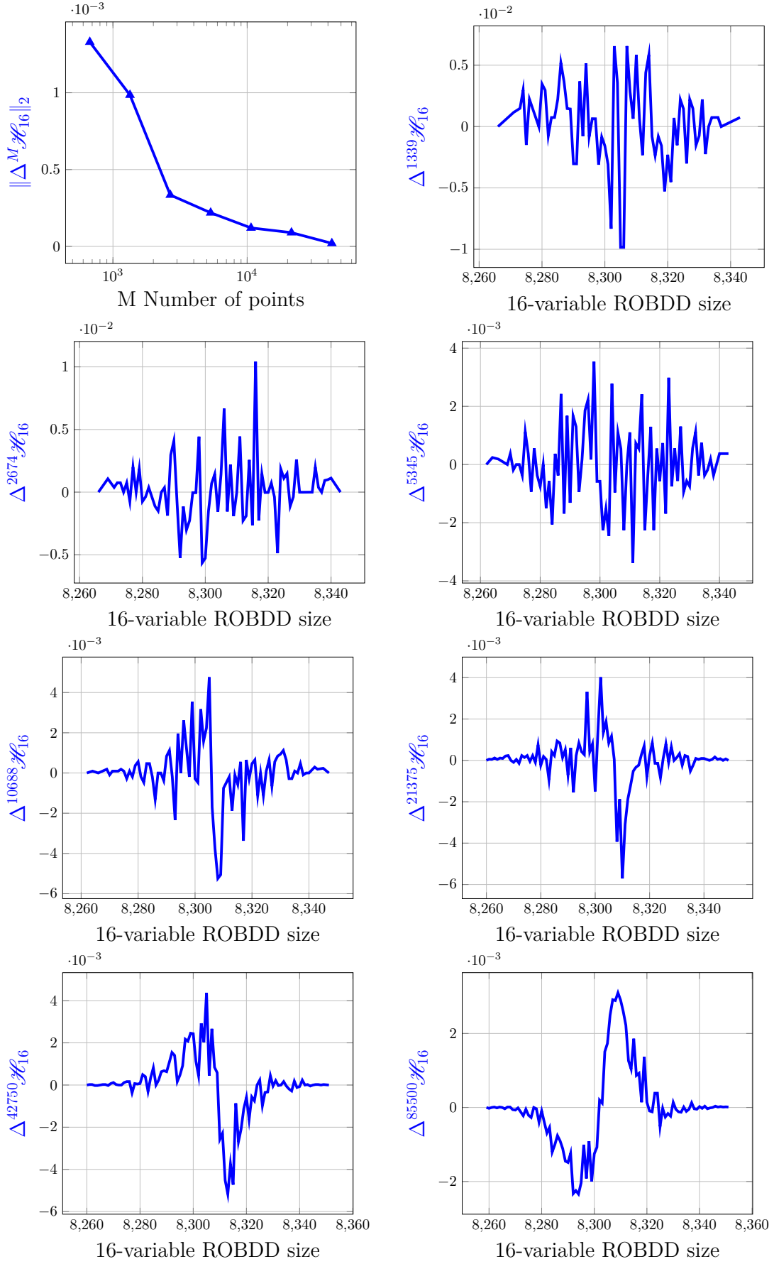
Figure 6.26: Difference functions for n = 16
