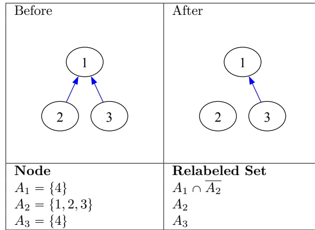
Figure 9.14: Connection between equal sets
