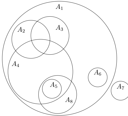
Figure 8.1: Venn Diagram of possibly overlapping sets. Each A_n is represented by a circle on this diagram.
