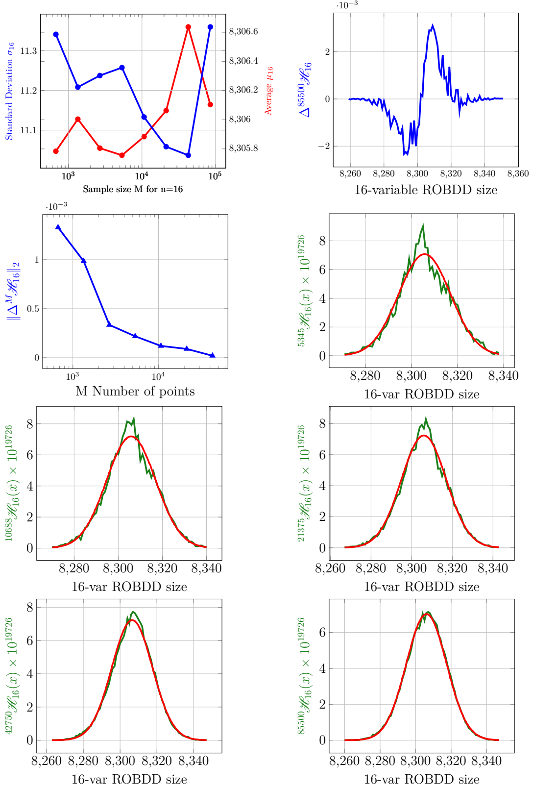
Figure 6.21: Histograms (from Figure 6.14) illustrating size distributions of successively larger samples for 16 variables, shown along with the theoretical normal distribution having the same \mu_{16} and \sigma_{16} . This figure also shows (top left) the plots of y = \mu_{16} and y = \sigma_{16} vs. x = node count for successively larger values of M . The plot in top right shows the difference function y = \Delta^M \mathcal{H}_{16} for the maximum sample size taken, M . Also shown in the plot of y = \|\Delta^M \mathcal{H}_{16}\|_2 for successively larger values of M which serves as an indicator of convergence of the \mathcal{H}_{16} curves.
