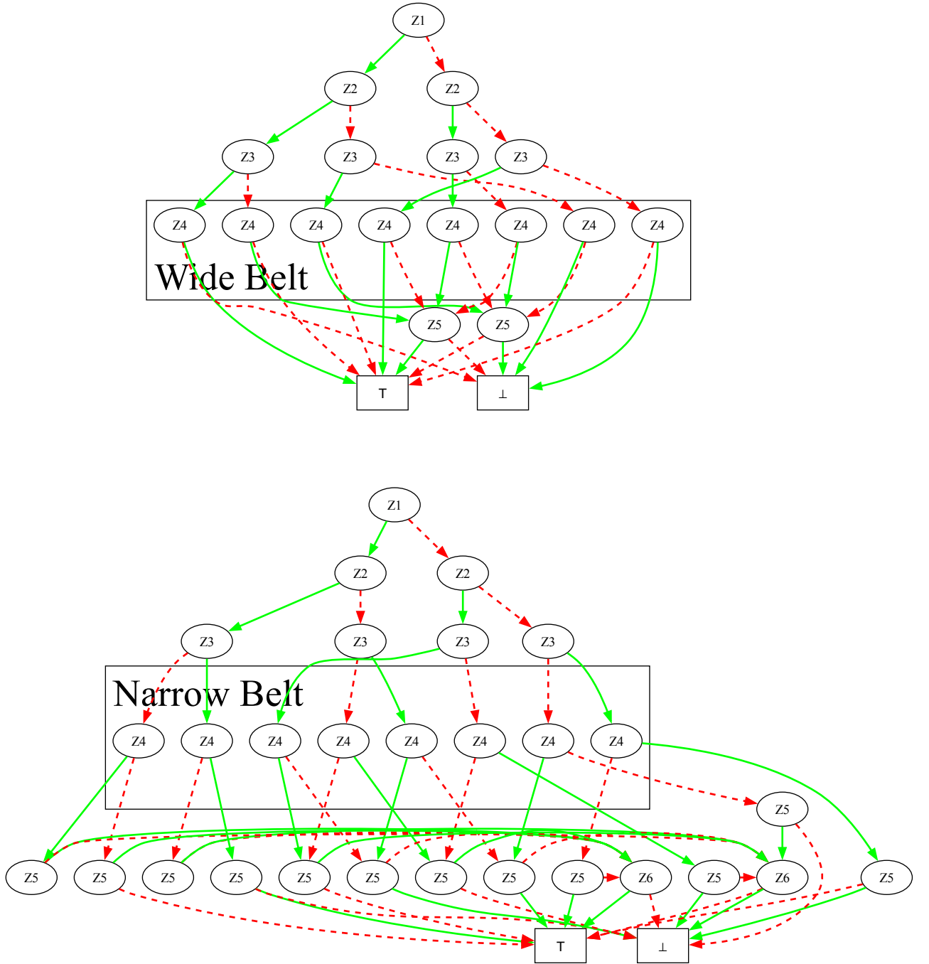
Figure 6.36: Belt connections of the ROBDD for 5 and 6 variables. The narrow belt only connects to the row directly below it. The wide belt connects not only to the row below it, but also to other, lower rows.
