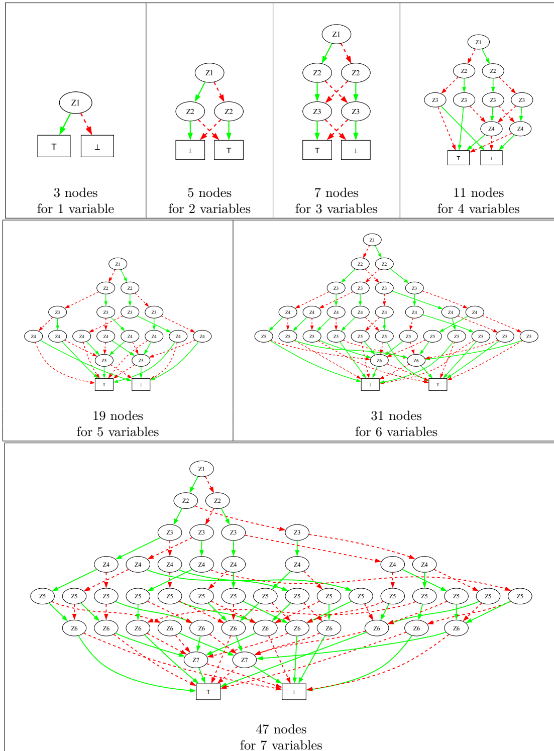
Figure 6.29: Shapes of worst-case ROBDDs for 1 to 7 variables
