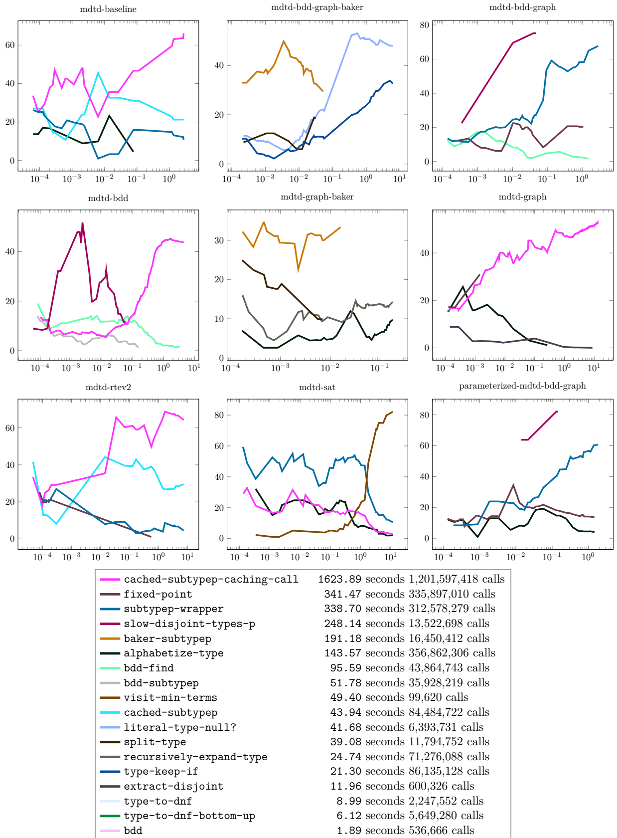
Figure 10.26: Performance Profile of various MDTD functions for pool Subtypes of CONDITION . Each plot is displayed with y='Profile Percentage' vs. x='Computation Time (seconds)'.
