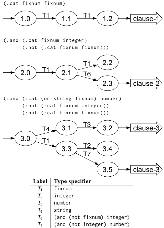
Figure 9: DFAs for disjoint clause-1, clause-2, and clause-3
