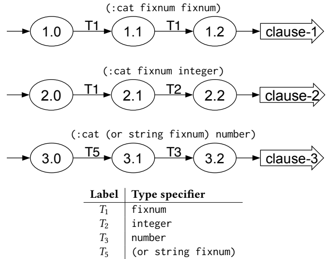
Figure 7: Automata for clauses of rte-case in Figure 2
