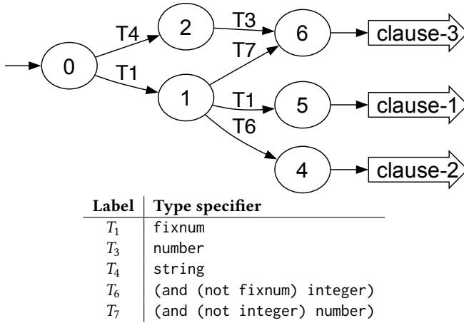
Figure 13: DFA for rte-case simplified
