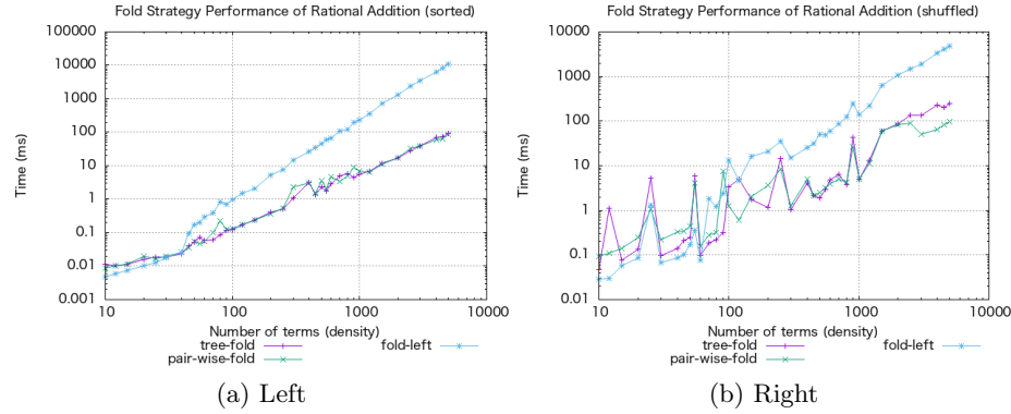
Fig. 4: Performance of fold strategy on rational addition. Left shows addition in sorted order. Right shows addition in randomized/shuffled order.
