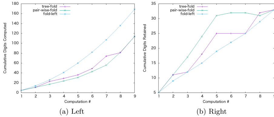
Fig. 3: (Left) Cumulative Digits Computed For Each Fold Strategy. (Right) Quantity of Digits Retained at each Computation State
