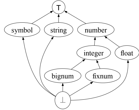
Figure 2: Example hierarchy of hosted types. Arrows point from subtype to supertype.
