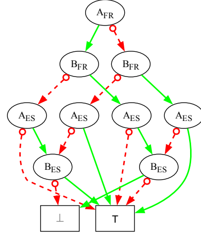
Figure 5.8: \text{FR} \rightarrow \text{ES} BDD representing France/Spain border. \text{FR} \rightarrow \text{DE} BDD of France/Germany border is isomorphic, but with different labels. (A_{\text{FR}}, B_{\text{FR}}) , (A_{\text{ES}}, B_{\text{ES}}) , and (A_{\text{DE}}, B_{\text{DE}}) are the colors of France, Spain, and Germany respectively.
