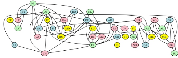
Figure 5.6: Coloring a map of some European countries
