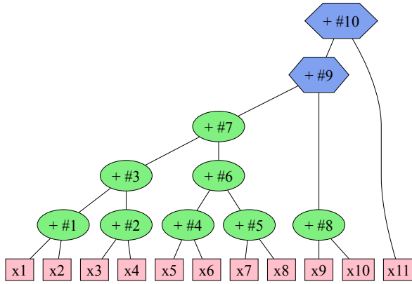
Figure 4.1: Intermediate and final values of adding 10 ratios, default fold-left algorithm, computed as shown in (10).
