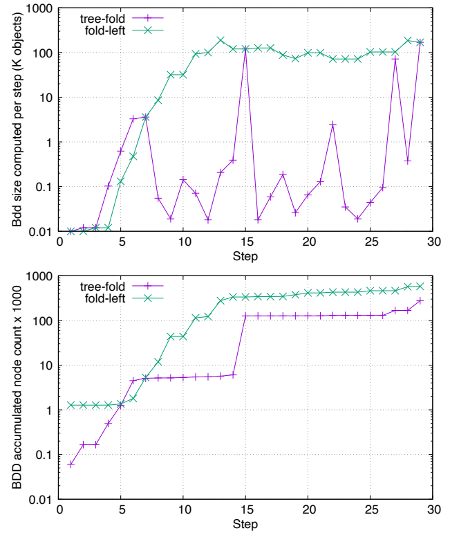
Figure 5.11: BDD node count. Top: Nodes allocated at each step of the iteration. Bottom: Total node accumulated thus far. Top is effectively the derivative of the bottom. Fewer nodes allocated is better than more.
