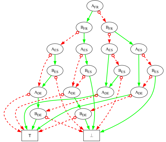
Figure 5.9: Two constraints corresponding to France/Spain and France/Germany
