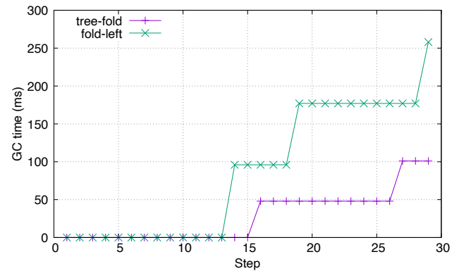
Figure 5.12: Time (milliseconds) spent in GC while coloring a map of Europe. Fewer milliseconds is better than more.
